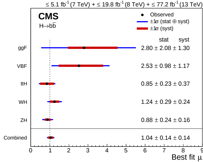
Figure 3: Best-fit value of the H \rightarrow b\bar{b} signal strength with its 1\sigma systematic (red) and total (blue) uncertainties for the five individual production modes considered, as well as the overall combined result. The vertical dashed line indicates the standard model expectation. All results are extracted from a single fit combining all input analyses, with m_H = 125.09 GeV.
