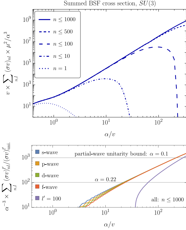
FIG. 2. Upper: the adjoint-to-singlet bound-state formation cross section in Eq. (6) shown for SU(3) , summed over all possible final bound-state quantum numbers n and \ell \leq n-1 . From the truncation of the sum for n \leq 1, 10, 100, 1000 (blue), one can infer that higher excited states contribute more for decreasing velocity. Lower: rescaled ratio of BSF cross section for fixed initial angular momentum \ell' and the corresponding partial-wave unitarity limit. For a given \alpha , unitarity is violated when the rescaled ratio is above 1/\alpha^3 , for which two examples are shown by the horizontal lines.
