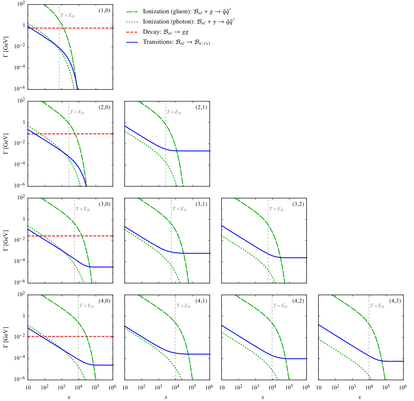
FIG. 5. Ionization, decay and transition rates for all bound state levels (n, \ell) up to n = 4 for m_{\tilde{q}} = 4 \times 10^6 GeV. The gray dashed vertical line indicates the temperature that corresponds to the binding energy E_B of the respective bound state. Note that the transition rates contain all possible excitations and deexcitations (here summed up to n' = 20 ).
