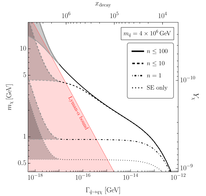
FIG. 9. Dark matter mass m_{\chi} and decay rate \Gamma_{\tilde{q} \rightarrow q\chi} of the colored t -channel mediator for which the final yield matches the observed dark matter density \Omega_{\chi} h^2 = 0.12 , using m_{\tilde{q}} = 4 \times 10^6 GeV. The abundance is set by the superWIMP mechanism for \Gamma_{\tilde{q} \rightarrow q\chi} \lesssim 10^{-13} GeV, while freeze-in dominates for larger decay rates. When taking only Sommerfeld-enhanced \tilde{q}\tilde{q}^{\dagger} annihilation into account (dotted line) the relic density is independent of \Gamma_{\tilde{q} \rightarrow q\chi} within the superWIMP regime, i.e., the dotted line is horizontal. The same is true when taking the ground state n = 1 into account (dot-dashed line). When including excited states, the mediator depletion due to BSF, transitions and decay of bound states continues until eventually H \sim \Gamma_{\tilde{q} \rightarrow q\chi} , such that the relic density does depend on the mediator lifetime, corresponding to the black dashed ( n \leq 10 ) and black solid ( n \leq 100 ) lines. For \Gamma_{\tilde{q} \rightarrow q\chi} \gtrsim 10^{-17} GeV the mediator decays before the QCD transition, i.e., within the perturbative regime. The shaded areas bracket the possible values for even lower decay rates, see text for details. The red shaded region is excluded at 95% C.L. by Lyman- \alpha forest observations [40].
