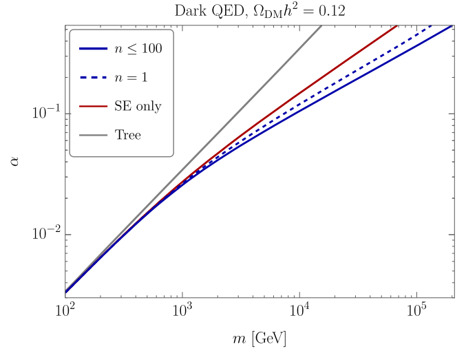
FIG. 10. Coupling strength \alpha versus the dark matter mass m shown for various approximations, imposing the right relic abundance constraint. Excited states with n \leq 100 , \ell \leq n - 1 and all dark electric dipole transitions among them (about a million) shown as the blue solid line, are a major correction to the original computation of capture into the ground state only on top of the Sommerfeld effect (blue dashed), cf., Ref. [18].
