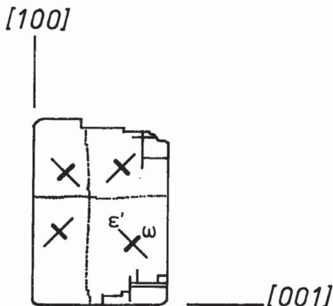
FIG. 1. Relation between cleavage, twinning and optical orientation for a thick grain of burtite resting on a cleavage plane. Indices refer to the individual in the lower right-hand corner. The plane of the drawing is (010) for that individual.
