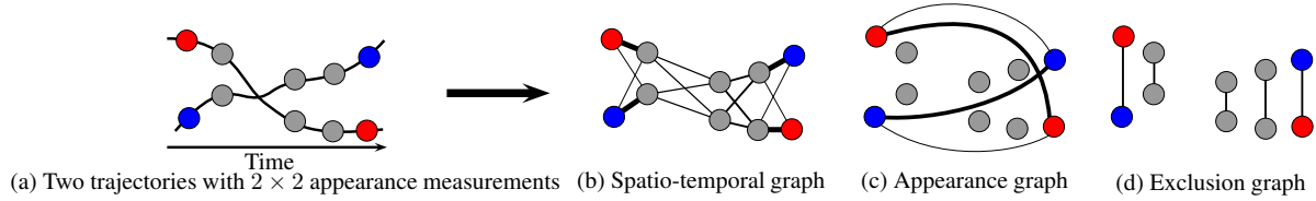
Figure 1. Best viewed in color. (a) An example with two targets (red and blue) with associated detections at each time. Gray detections mean that no appearance feature is available. (b) Spatio-temporal graph that depicts the spatio-temporal association between the nodes, (c) Appearance graph that connects nodes even if they are far in time. (d) Exclusion graph in which edges connect nodes that coexist at the same time. In graphs (b) and (c), thickness of an edge is proportional to its weight.
