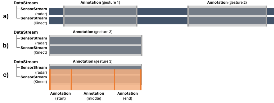
Fig. 1.6: Illustration of DataStreams, SensorStreams, and Annotations: a) a DataStream containing two gestures delimited using annotations, b) one gesture spanning the entire DataStream, c) a gesture with sub-annotations delimiting its start, middle, and end.
