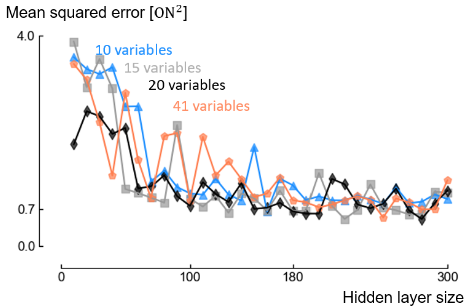
Figure 3: MSE with the B2 and the Auto methods. The MSE decreases with the size of the hidden layer. Moreover, the MSE increases when the number of selected variable decreases. Therefore, the variable selection method B2 is not appropriate.
