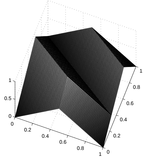
Sequential-Merge inequality with r_1 = 0.5, r_2 = 0.25
