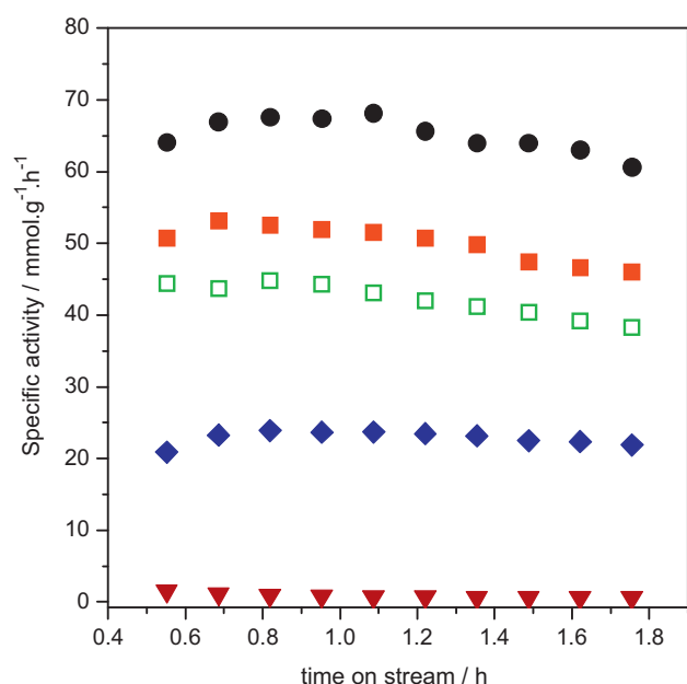
Fig. 6. Specific activity (mmol of propene produced per g of catalyst and per hour) with time on stream over (●) WO x /SiAl-aer, (■) WO x -impSiAl-aer, (□) WO x -imp-SiAl, (◆) WO x -imp-Al, (▼) WO x -imp-Si.
