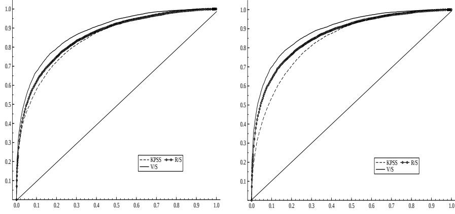
Figure 3: Gegenbauer Process: d = 0.15 , \hat{\sigma}_{V_{BIC}}^2 , n = 500 , \cos \omega = 0.99999 (left) and \cos \omega = 0.9999 (right)
