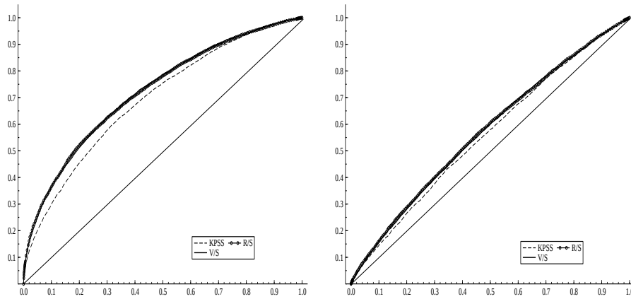
Figure 2: Semi LARCH(1, d ,1) Process: d = 0.30 , \hat{\sigma}_{V_{BIC}}^2 , n = 500 , r = 0.99 (left) and r = 0.9 (right)
