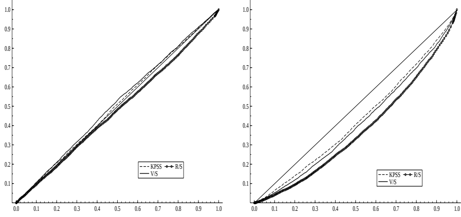
Figure 4: Gegenbauer Process: d = 0.15 , \hat{\sigma}_{V_{BIC}}^2 , n = 500 , \cos \omega = 0.99 (left) and \cos \omega = 0.95 (right)
