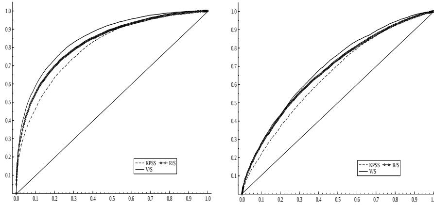
Figure 1: Semi Farima Process: d = 0.30 , \hat{\sigma}_{V_{BIC}}^2 , n = 500 , r = 0.99 (left) and r = 0.9 (right)
