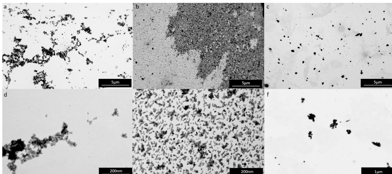
Fig. 4. Transmission electron microscope (TEM) images for (a & d) ZnO A, (b & e) ZnO B, and (c & f) ZnO C.
