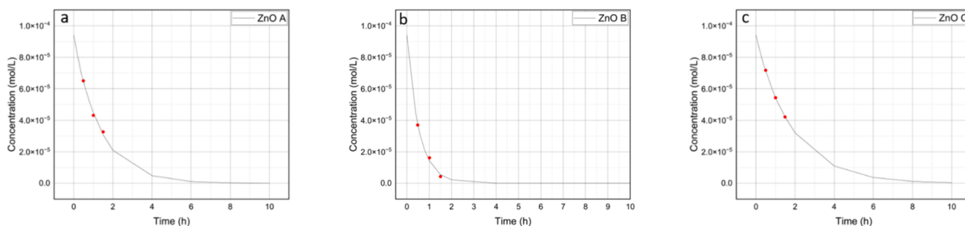
Fig. 8. Curves derived from k values and equation (4) (black) and experimental points for p-nitrophenol (PNP) degradation (red) after 30, 60, and 90 min under UV-A for (a) ZnO A, (b) ZnO B, and (c) ZnO C. (For interpretation of the references to colour in this figure legend, the reader is referred to the web version of this article.)
