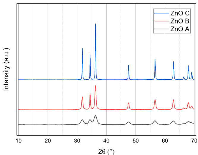
Fig. 1. X-ray diffraction patterns for the three powders: ZnO A (black), ZnO B (red), and ZnO C (blue). (For interpretation of the references to colour in this figure legend, the reader is referred to the web version of this article.)
