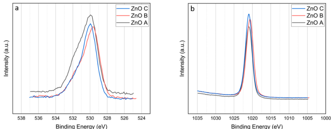
Fig. 6. (a) O1s and (b) Zn2p spectra for the three catalysts ZnO A (black), ZnO B (red), and ZnO C (blue). (For interpretation of the references to colour in this figure legend, the reader is referred to the web version of this article.)
