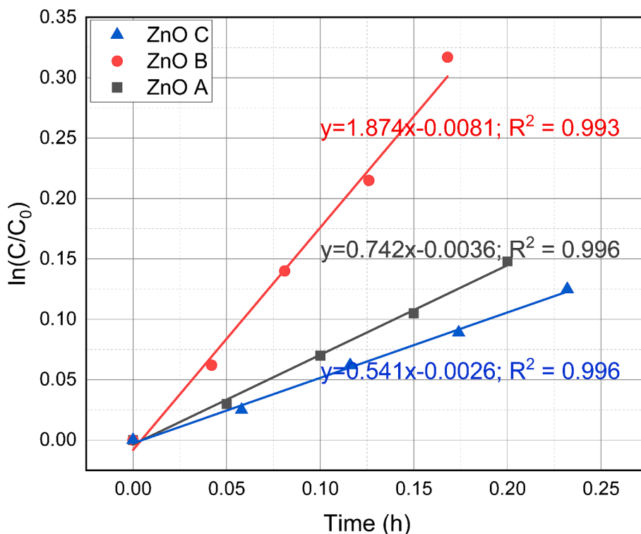
Fig. 7. Experimental determination of kinetic constant k of catalyst-mediated degradation by sampling 1 mL of p-nitrophenol (PNP) solution at 4 different times. In grey, ZnO A; red, ZnO B; blue, ZnO C. (For interpretation of the references to colour in this figure legend, the reader is referred to the web version of this article.)
