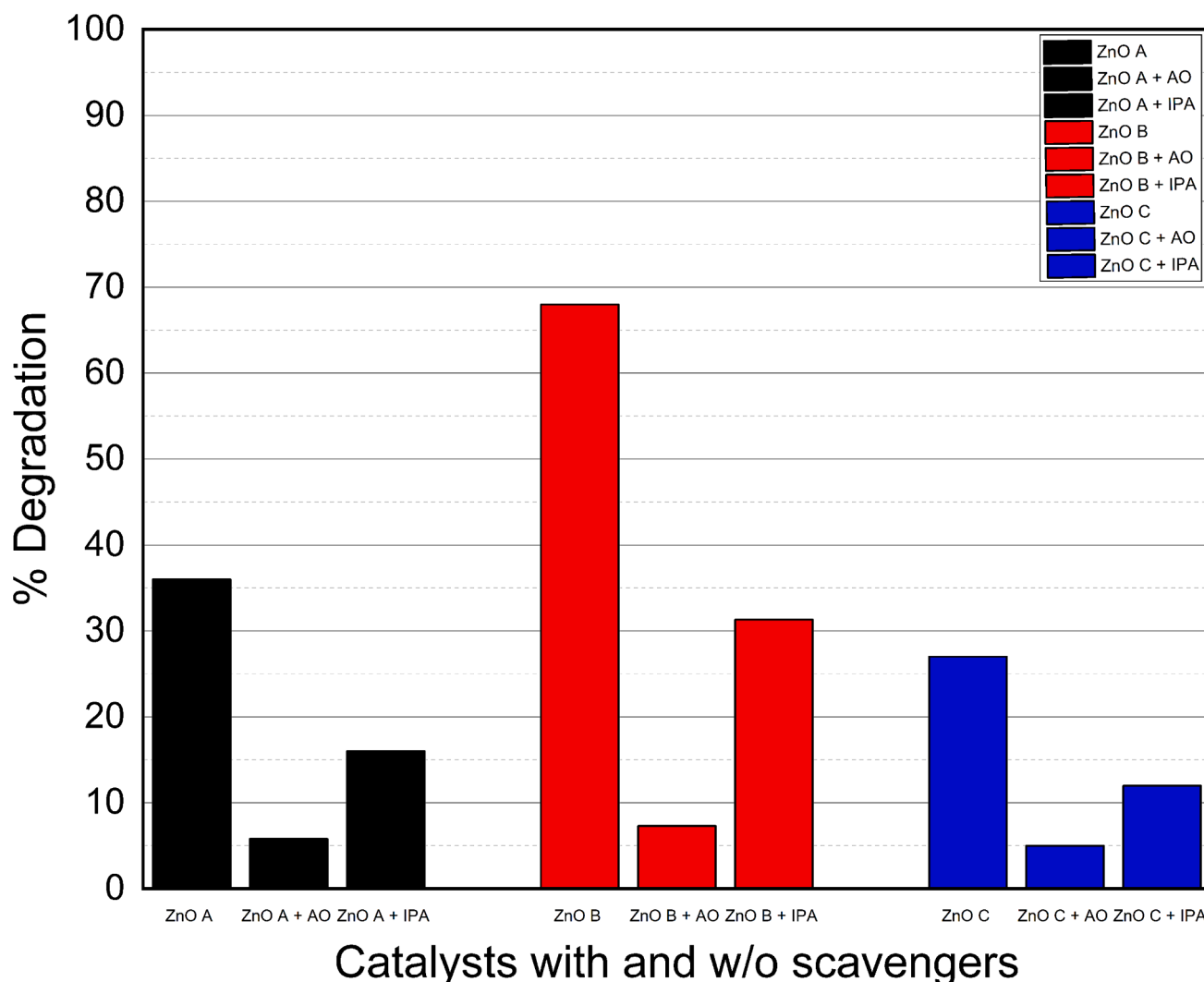
Fig. 9. Degradation of p-nitrophenol (PNP) by the three catalysts (ZnO A, B, and C) with and without scavenger during 30 min under UV-A illumination. AO = ammonium oxalate, IPA = isopropanol.
