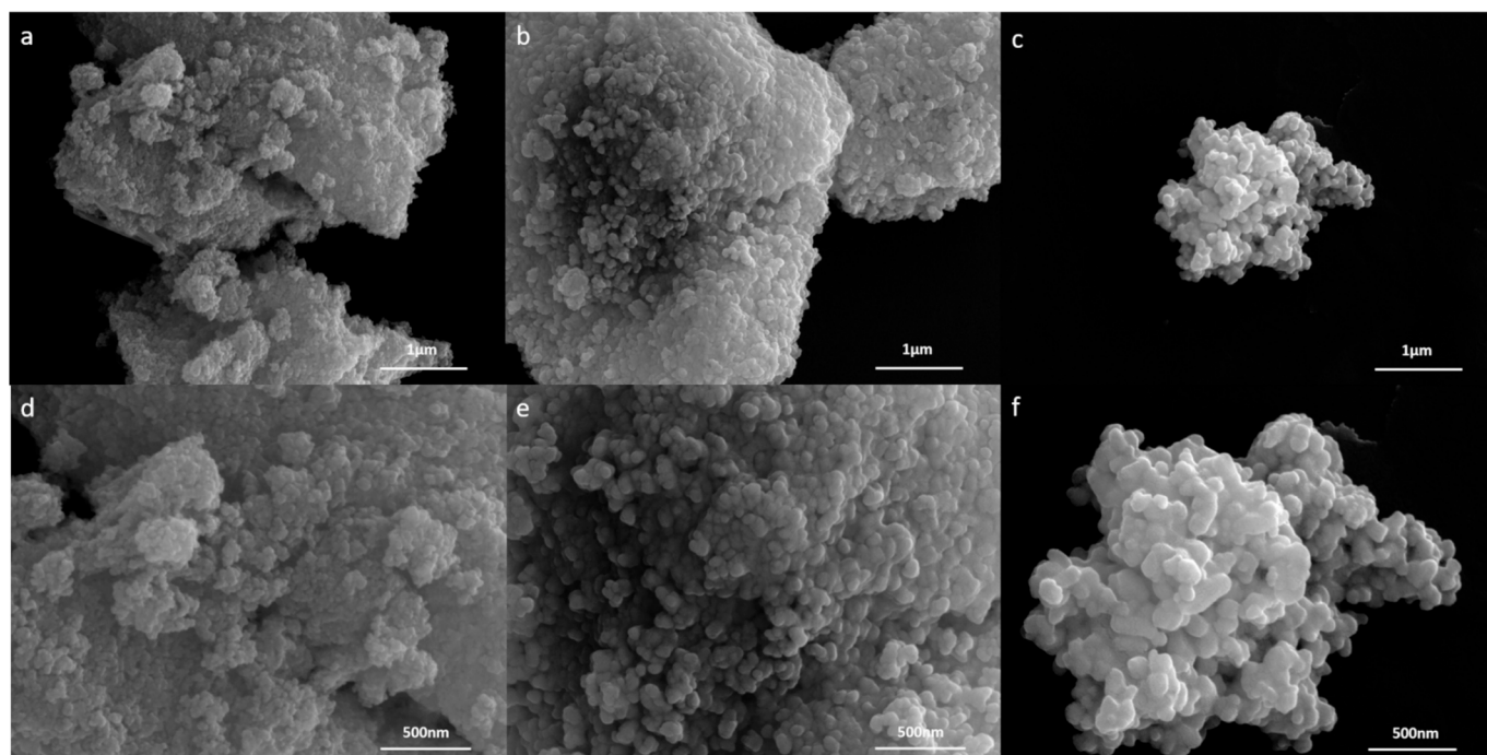
Fig. 3. Scanning electron microscope (SEM) images for the three different catalysts at a magnification of 50000 \times and 100000 \times : (a, d) ZnO A; (b, e) ZnO B; (c, f) ZnO C.
