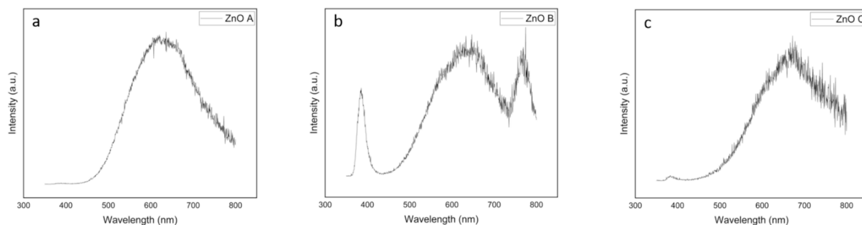
Fig. 5. Photoluminescence (PL) spectra ( \lambda_{\text{exc}} = 325 nm) for the three ZnO samples: (a) ZnO A, (b) ZnO B, and (c) ZnO C.
