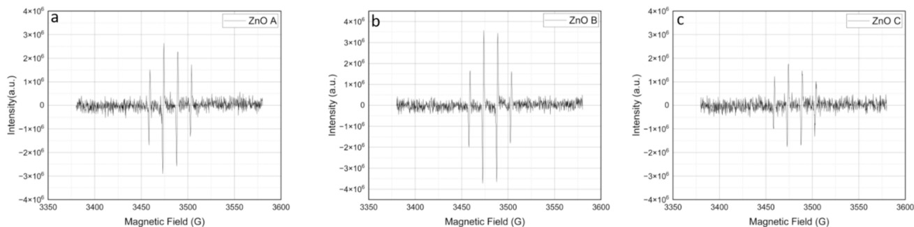
Fig. 10. Electron paramagnetic resonance (EPR) spectra for the three catalysts (ZnO A, B, and C) with 5,5-dimethyl-1-pyrroline-N-oxide (DMPO). Spectra are recorded after UV-A illumination for 150 s with DMPO and catalysts at a concentration of 1 g/L.
