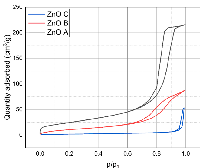
Fig. 2. Nitrogen adsorption-desorption isotherms for the three samples, from top to bottom: ZnO A (black), ZnO B (red), ZnO C (blue). (For interpretation of the references to colour in this figure legend, the reader is referred to the web version of this article.)
