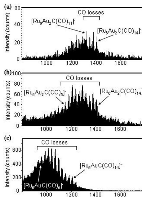
Figure 2. Negative SIMS spectra of the cluster [Ru_6Au_2C(CO)_{12}-(PPh_3)_2] (2) before thermal treatment: (a) pure unsupported cluster as reference, (b) cluster 2 deposited onto C_{SX+} and (c) cluster 2 anchored onto C_{PPh_2} .
