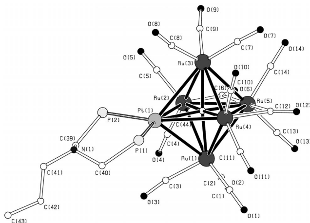
Figure 5. Molecular X-ray structure of the cluster [\text{Ru}_5\text{PtC}(\text{CO})_{14}\{(\text{PPh}_2\text{CH}_2)_2\text{NC}_3\text{H}_7\}] ( 4 ) obtained by X-ray crystallography; Ph groups are omitted for clarity.
