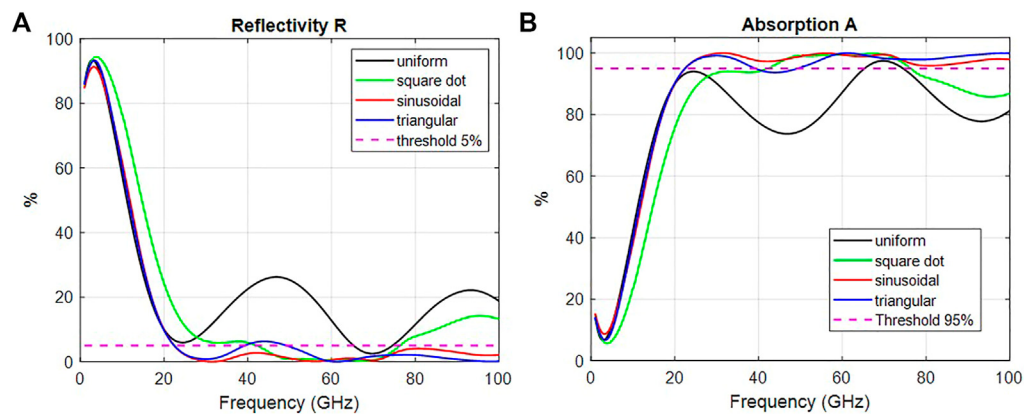
FIGURE 3 Performances of profiles of Figure 1 (A) reflectivity R (B) absorption A.
