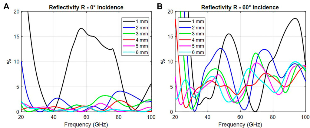
FIGURE 6 Reflectivity R for various heights h of the unit cell (A) 0^\circ incidence (B) 60^\circ incidence.
