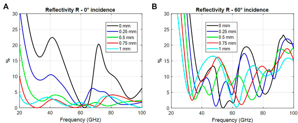
FIGURE 7 Reflectivity R for various heights h_s of the support layer (A) 0^\circ incidence (B) 60^\circ incidence.
