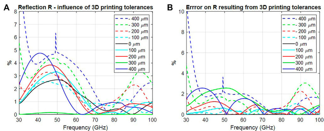
FIGURE 11 (A) Influence of 3D manufacturing tolerances on reflectivity R (B) Error on R.
