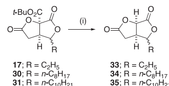
Scheme 5. Krapcho decarboxylation. (i) LiCl, DMSO, water, 160 °C, 1 h; 33 , 80%; 34 , 77%; 35 , 96%.
