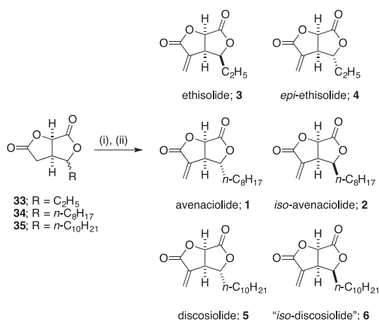
Scheme 6. Synthesis of the natural products. (i) CH 3 OMgOCO 2 CH 3 (Stile's reagent), DMF, 120 °C; (ii) H 2 CO, H 2 O, Et 2 NH, NaOAc, AcOH, RT then 100 °C; 3 18%, 4 34%; 1 34%, 2 26%; 5 28%, 6 10%.
