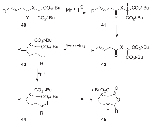
Scheme 8. Plausible mechanism of the oxidative lactonization reaction. X = Y = O or X = CH 2 , Y = H 2 .
