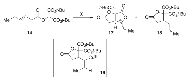
Scheme 3. Oxidative radical cyclization. (i) Mn(OAc) 3 , Cu(OTf) 2 , MeCN, 40 °C, 17 24% (1.2:1 mixture of C-4 diastereomers), 18 40% (3.8:1 mixture of (E):(Z) diastereomers).
