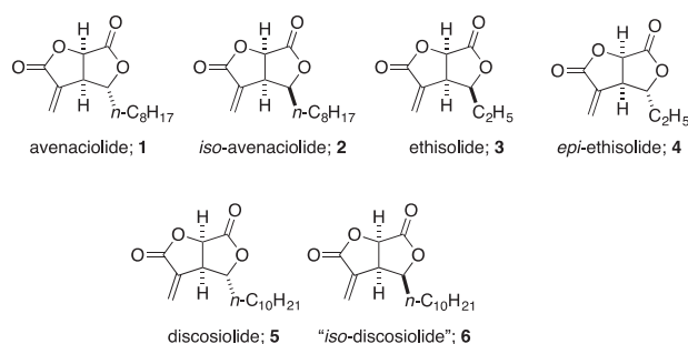
Fig. 1. \alpha -Methylene- \gamma -lactone natural products of the avenaciolide family.
