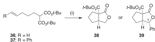
Scheme 7. Synthesis of carbocyclic products. (i) Mn(OAc) 3 , KI, MeCN, 80 °C, 21 h; 38 46%; 39 88% (9:1 mixture of C-1 diastereomers, major diastereomer shown).
