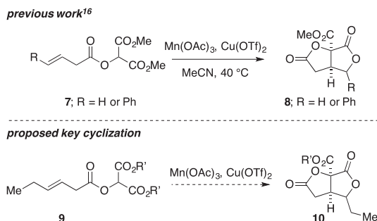
Scheme 1. Oxidative radical cyclization to form bis-lactones.
