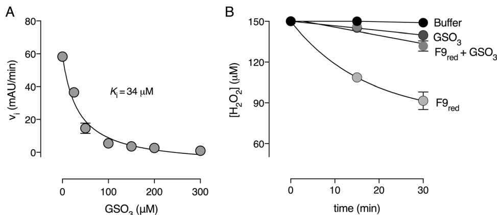
Figure 5. Glutathione sulfonate ( \text{GSO}_3 ) inhibits GSTF9 glutathione transferase and peroxidase activity. Increasing concentrations of \text{GSO}_3 results in a decrease of the initial velocity of (A) the GSTF9 glutathione transferase and (B) the peroxidase activity. The inhibition constant ( K_i ) for the transferase activity is 34 \mu\text{M} . The data represent the mean \pm SD of 2 independent experiments.
