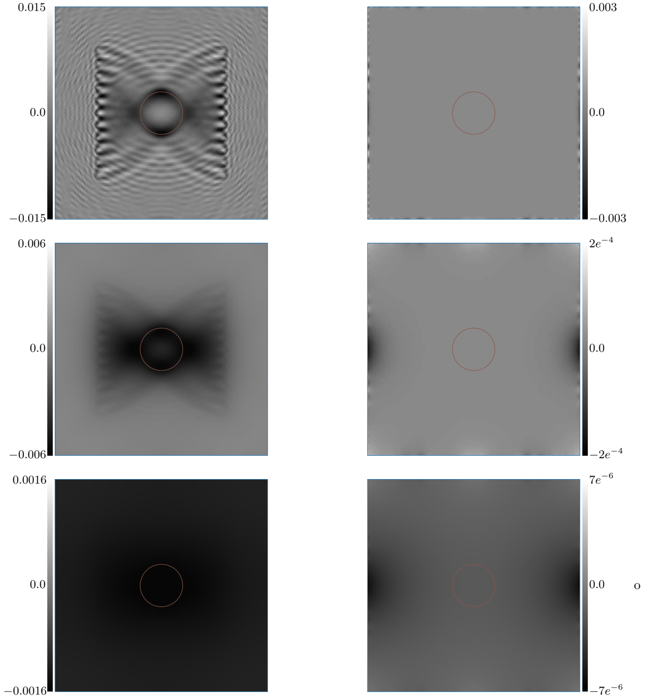
Figure 8: Bulk (left column) and boundary (right column) parts of the H_1 -Sobolev gradient for several values of the smoothing length l_c := 2\pi\sqrt{\alpha_1} ; l_c = 1 (top row), l_c = 10 (middle row), l_c = 100 (bottom row). The data used for this gradient is obtained with a highly penetrable cylinder ( \tilde{s}_0^2 = 1.0 and \tilde{s}_c^2 = 1.2 ).
