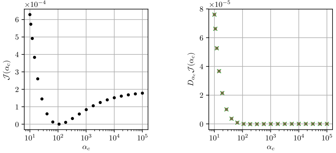
Figure 5: Performance functional (●) and its derivative for a weakly penetrable cylinder whose penetrability \alpha_c varies around the true value \bar{\alpha}_c = 100 . The derivatives are computed by the adjoint state method (○) and by an approximation of the definition (3)(with \epsilon = 10^{-5} ) (×).
