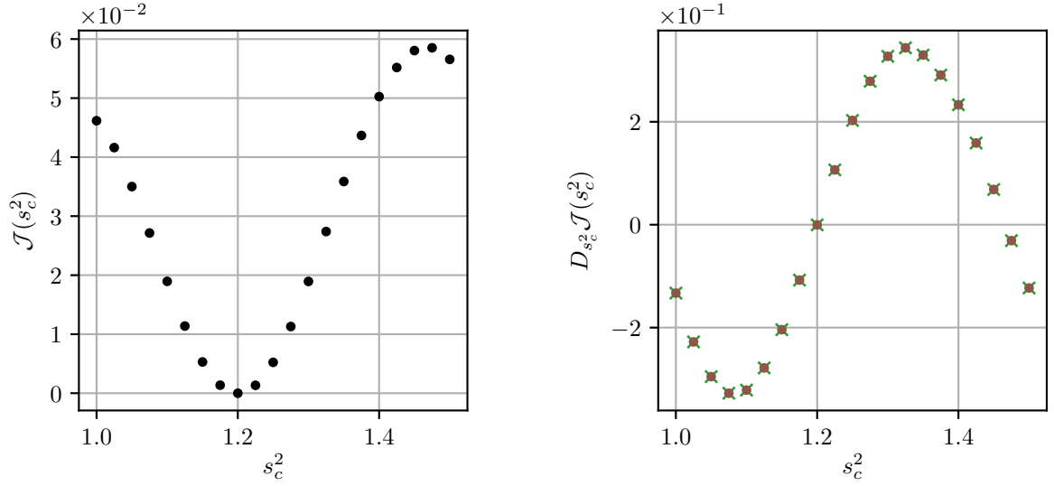
Figure 3: Performance functional ( \bullet ) and its derivative for a highly penetrable cylinder whose slowness squared s_c^2 varies around the true value \tilde{s}_c^2 = 1.2 . The derivatives are computed by the adjoint state method ( \bullet ) and by an approximation of the definition (3) (with \epsilon = 10^{-5} ) ( \times ).
