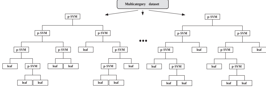
Fig. 1: Embedded proximal SVMs in an ensemble of decision trees
