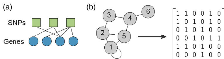
FIGURE 1 (a) A bipartite graph, in this case showing eQTL associations. (b) A unipartite graph and its corresponding adjacency matrix
