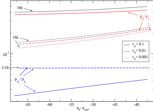
FIG. 13: Ratios between the power spectra of Fig. 11 and their evolution with respect to the moduli coupling constant c_p . The “consistency check” \mathcal{P}_h/\mathcal{P}_\zeta = 16e is recovered in the weak coupling limit while significant deviations appear for c_p = 0.1 due to the sourcing effects between the modes after Hubble exit.
