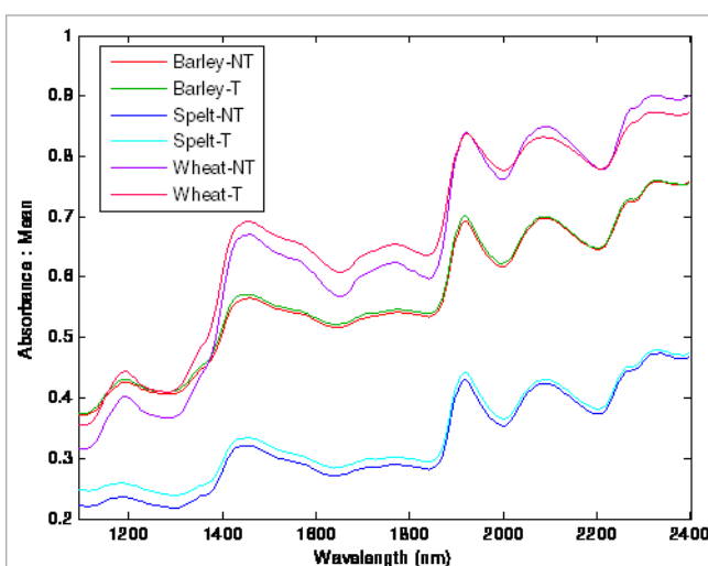
Figure 2. NIR-HSI spectra of treated (T) and not treated (NT) seeds from wheat, barley and spelt.
