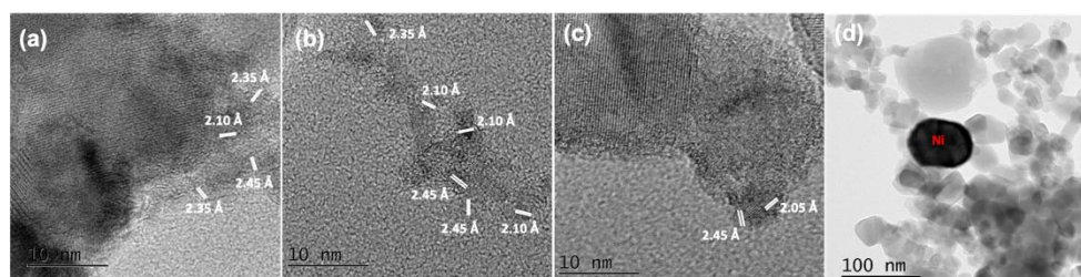
Figure 3. TEM images of (a) and (b) the as-prepared Ni/TiO 2 catalyst and (c) and (d) the spent Ni/TiO 2 catalyst.
