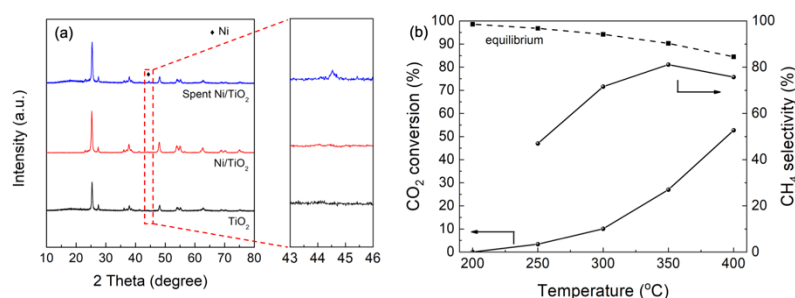
Figure 2. (a) XRD patterns of the TiO 2 support, as-prepared Ni/TiO 2 catalyst and spent Ni/TiO 2 catalyst. (b) CO 2 conversion and CH 4 selectivity of Ni/TiO 2 catalyst as a function of temperature.
