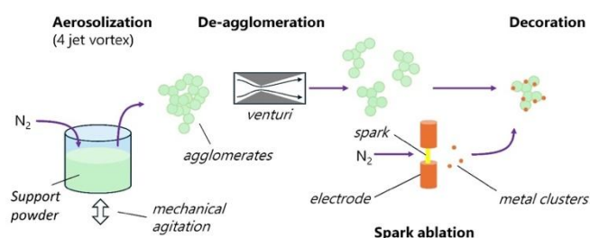
Figure 1. Schematic view on the set-up used to prepare powdery Ni/TiO 2 and Ru/TiO 2 catalysts.
