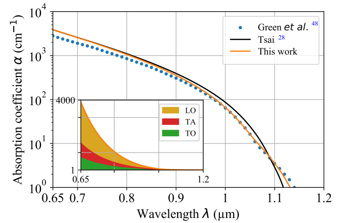
FIG. 2. Comparison between our indirect absorption coefficient computed including the contributions of the TA, TO and LO modes (solid orange line) with that obtained by Tsai, including only the TO and TA modes with different parameters (solid black line). These are compared with the absorption coefficient measured experimentally by Green et al. (blue circles). 48 The inset shows the contributions of the TA, TO and LO modes to the absorption coefficient.
