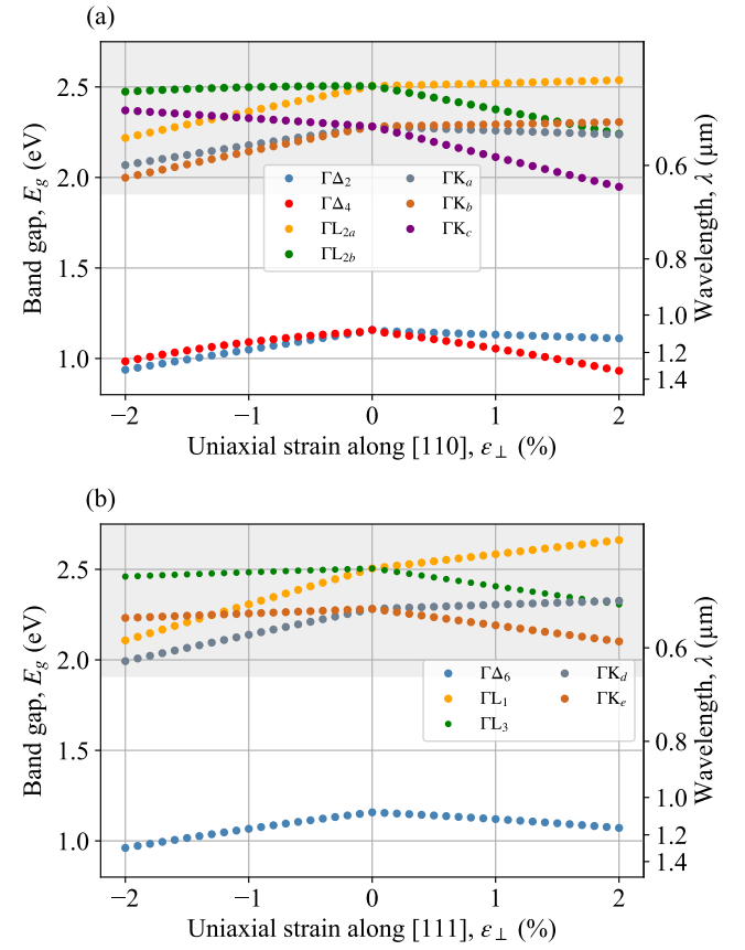
FIG. 5. Evolution of the indirect band gaps of silicon with a uniaxial strain applied along the (a) [110] and (b) [111] directions. The gray shaded zone denotes energies outside the region of interest.
