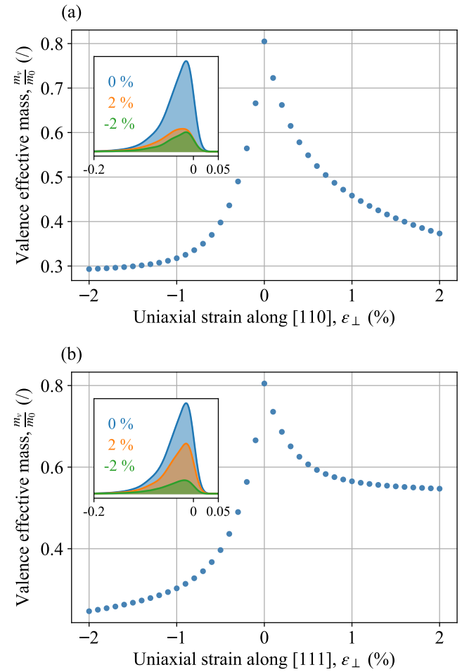
FIG. 7. Evolution of the valence band density-of-states effective mass with a uniaxial strain applied along the (a) [110] and (b) [111] directions.
