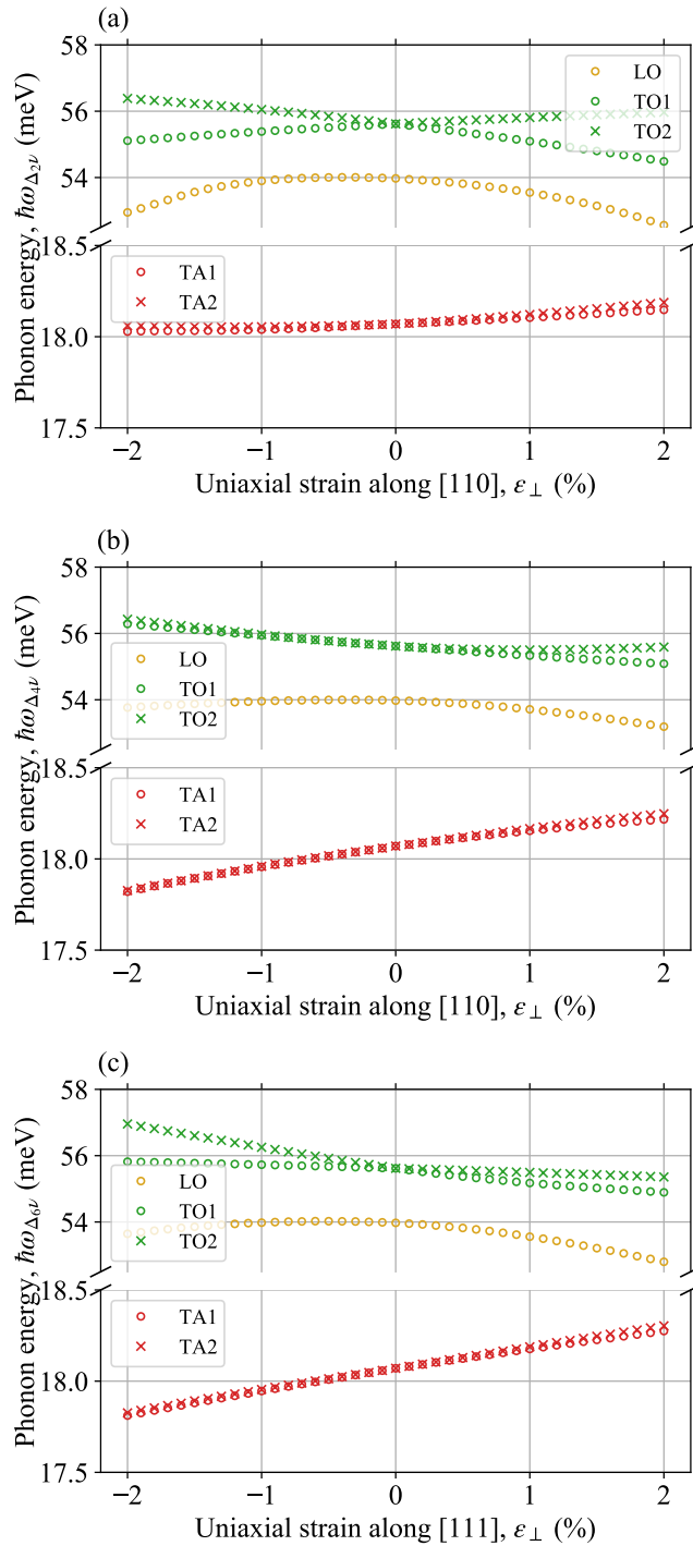
FIG. 8. Evolution of the optical and acoustic phonons energies at (a) the \Delta_2 and (b) the \Delta_4 valleys under uniaxial [110] strain, and (c) the \Delta_6 valleys under uniaxial [111] strain.
