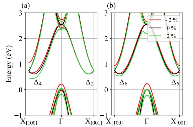
FIG. 3. Electronic DFT band structure of relaxed (black) and highly strained silicon, along different \Gamma – X directions. A uniaxial strain of -2\% (red) and +2\% (green) is applied along the (a) [110] and (b) [111] directions. The zero of energy is set at the valence band maximum in the relaxed case.
