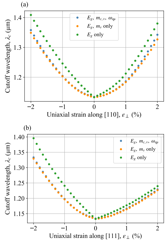
FIG. 11. Evolution of the cutoff wavelength with a uniaxial strain applied in the (a) [110] and (b) [111] directions. Only the band gap changes with the strain are included (green), the valence band effective mass changes are also included (orange), or both effective masses and the phonon frequencies changes are also included (blue).
