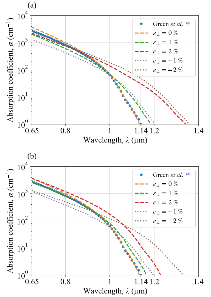
FIG. 9. Absorption coefficient spectrum of silicon for different uniaxial strain levels in the (a) [110] and (b) [111] directions.
