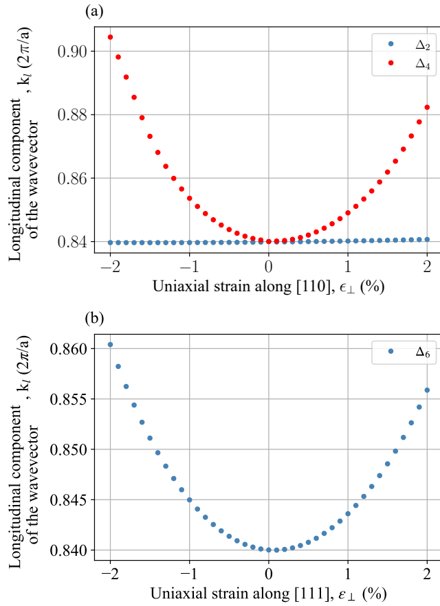
FIG. 4. Evolution of the longitudinal component of the \Delta -valley wavevector (in units of 2\pi/a , with a the unit cell parameter) with a uniaxial strain applied along the (a) [110] and (b) [111] directions.
