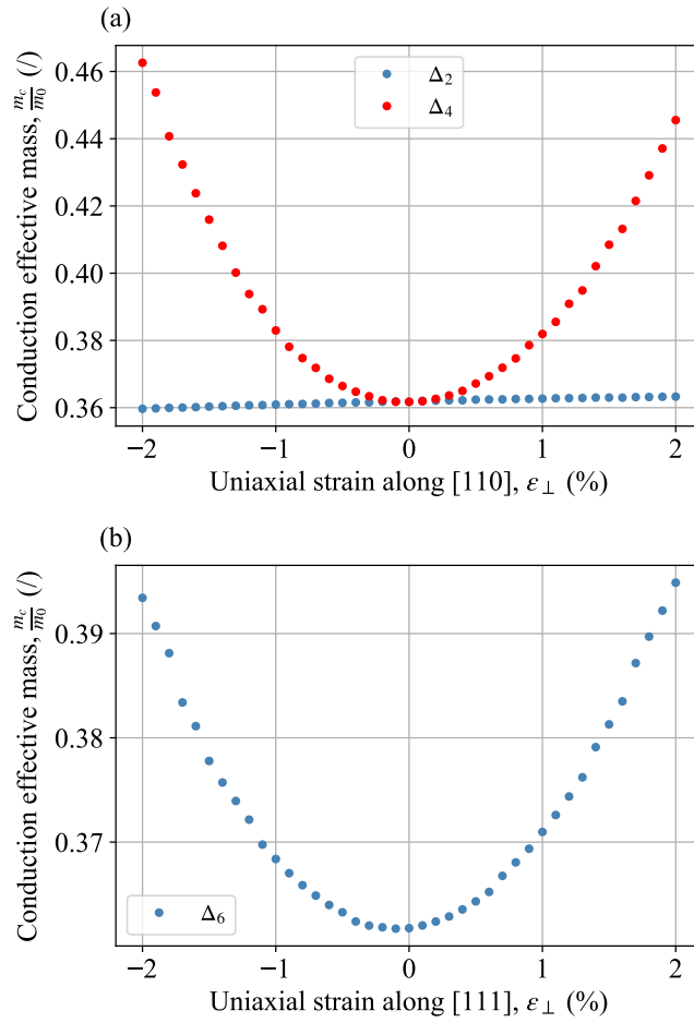
FIG. 6. Evolution of the conduction band density-of-states effective masses with a uniaxial strain applied along the (a) [110] and (b) [111] directions.
