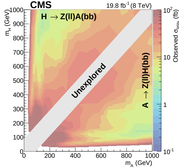
Figure 1: Observed 95% CL upper limits on \sigma_{H/A \rightarrow Z\ell\ell/A/H \rightarrow \ell\ell b\bar{b}} as a function of m_A and m_H .
