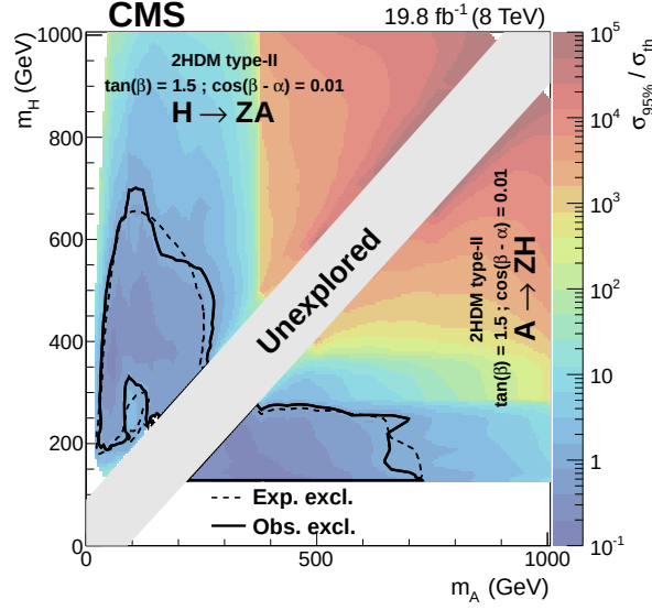
Figure 5: Observed limits on the signal strength \mu = \sigma_{95\%}/\sigma_{\text{th}} for the 2HDM benchmark, after combining results from \ell\ell b\bar{b} and \ell\ell\tau\tau final states. The cross sections are normalised to the NNLO SUSHi prediction, for a 2HDM type-II scenario with \tan\beta = 1.5 and \cos(\beta - \alpha) = 0.01 . The dashed contour shows the region expected to be excluded. The solid contour shows the region excluded by the data.
