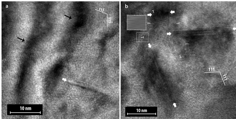
Fig. 3. HRTEM micrographs showing (a) FIB induced parallel dislocations indicated by black arrows from area A, and (b) nanoscale planar defects (white arrows) and some edge dislocations (⊥ mark) in area B.
