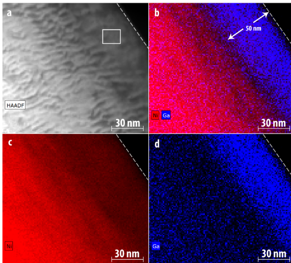
Fig. 4. (a) HAADF-STEM image, the Ga amount in the selected white rectangle is 10 \pm 1 at.% (using camera length of 330 nm still showing some dislocation contrast), (b) superposed HAADF-STEM image, Ni and Ga EDX chemical maps, (c) Ni EDX chemical map, and (d) Ga EDX chemical map.
