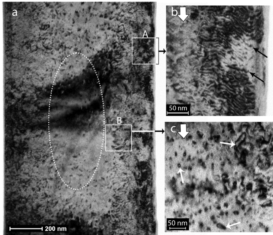
Fig. 2. (a) BF micrograph of sample before deformation, with highlighted regions A and B near the edges. (b) and (c) BF micrographs taken in two-beam condition with g = 11\bar{1} (large white arrows) from area A containing tangled dislocation structure (black arrows) and area B containing different size dislocation loops (small white arrows), respectively.
