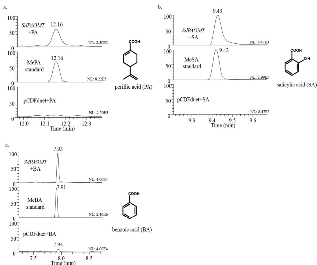
Fig. 6. Characterization of S. dorisiana O-methyltransferase SdPAOMT . Shown are GC-MS chromatograms of in vitro assays with different substrates. (a) SdPAOMT +perillid acid (PA), m/z=67.50-68.50 + 120.50-121.50 + 179.50-180.50 MS. (b) SdPAOMT +salicylic acid (SA), m/z=151.50-152.50 MS. (c) SdPAOMT +benzoic acid (BA), m/z 76.50-77.50 + 104.50-105.50 + 135.50-136.50 MS. pCDFduet empty vector control.
