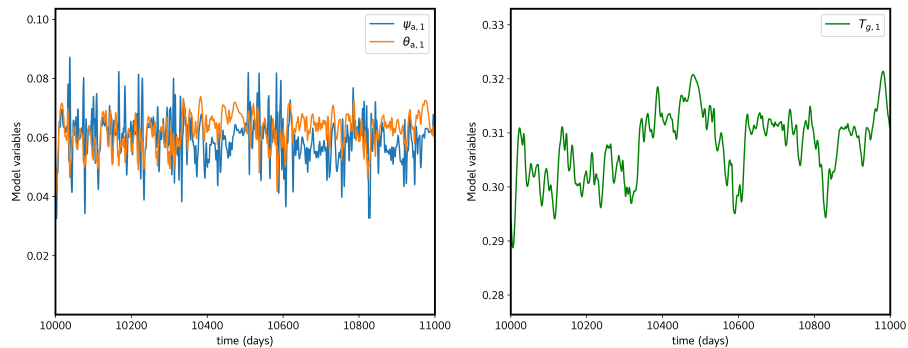
Figure 1. Temporal evolution of barotropic ( \psi_{a,1} ) and baroclinic ( \theta_{a,1} ) atmospheric streamfunction and the ground temperature ( T_{g,1} ) for C_g = 300 \text{ Wm}^{-2} and k_d = 0.085 .
