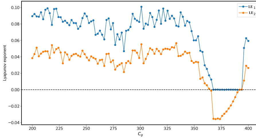
Figure 6. First and second Lyapunov exponents of the land atmospheric coupled model for different values of C_g for a fixed value of k_d = 0.08 . blue line represents first and orange line represents second Lyapunov exponents respectively. The values of the Lyapunov exponents are given in days -1
