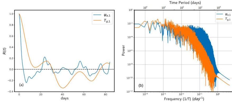
Figure 2. (a) Autocorrelation of barotropic ( \psi_{a,1} ) atmospheric streamfunction and the ground temperature ( T_{g,1} ) for C_g = 300 \text{ Wm}^{-2} and k_d = 0.085 . (b) Powerspectrum of the same variables.
