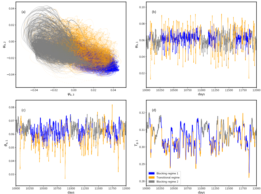
Figure B4. Phase space dynamics of the model projected on the (\psi_{a,3}, \psi_{a,2}) -plane is shown in panel (a) for k_d = 0.08 . The figure illustrates the Gaussian mixture clustering results, where each data point is colored according to its corresponding cluster or flow regime. Panels (b), (c), and (d) depict the temporal evolution of barotropic ( \psi_{a,1} ) and baroclinic ( \theta_{a,1} ) atmospheric streamfunction, along with ground temperature ( T_{g,1} ) for C_g = 300 \text{ Wm}^{-2} and k_d = 0.08 , with colors corresponding to their respective clusters.
