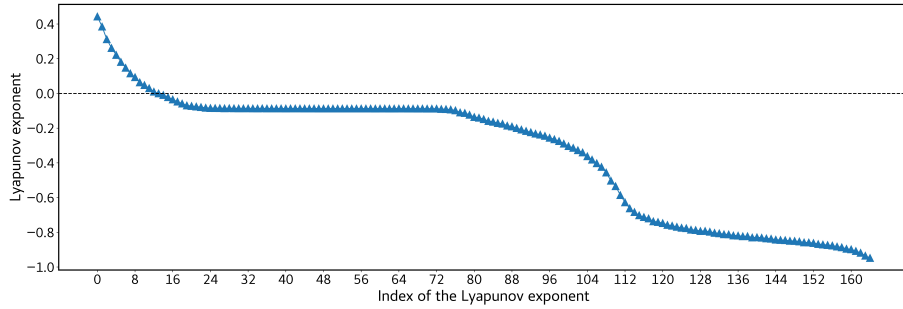
Figure 12. Lyapunov spectrum of the land-atmosphere coupled model for C_g = 300 \text{ Wm}^{-2} and k_d = 0.085 in (5,5) model configuration. The values of the Lyapunov exponents are given in days ^{-1} .
