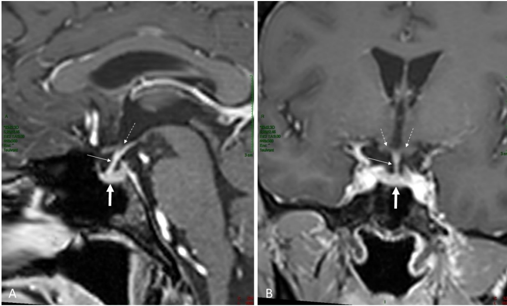
Figure 2. Magnetic resonance MR examination of Patient 1 at the time of DI. Reformated views from high-resolution post-contrast 3D T1-weighted volume (voxel size 1 mm 3 isotropic). A: mid-sagittal view showing normal pituitary gland (thick arrow), pituitary stalk (thin arrow), and infundibular recess (dotted arrow). B: coronal view confirming unremarkable gland (thick arrow) and stalk (thin arrow) together with normal hypothalamus (between dotted arrows).
