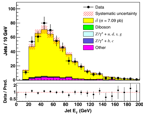
FIG. 1 (color online). Distribution of jet E_T values for the two jets with largest E_T in each event (black points) for the signal sample. The histogram represents the sum of the signal and background estimates, where the signal is normalized to the observed cross section. The hatched area is the total uncertainty on the sum of the signal and background predictions. The lower panel shows the observed data yield divided by the predicted yield.
