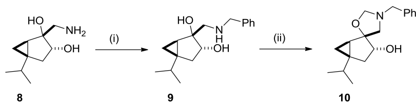
Scheme 2. Reagents and conditions: (i) PhCHO, dry EtOH, 2 h, then \text{NaBH}_4 , EtOH, 48 h, rt, 56%; (ii) 35% aq \text{CH}_2\text{O} , \text{Et}_2\text{O} , rt, 1 h, 90%.
