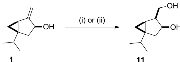
Scheme 3. (i) \text{BH}_3 \cdot \text{THF} , THF, 0^\circ\text{C} to rt, 2.5 h, then \text{NaOH}/\text{H}_2\text{O}_2/\text{H}_2\text{O} , THF, rt, 30 min, 47%; (ii) \text{BH}_3 \cdot \text{Me}_2\text{S} , THF, 0^\circ\text{C} to rt, 18 h, then \text{NaOH}/\text{H}_2\text{O}_2/\text{H}_2\text{O} , THF, rt, 30 min, 70%.
