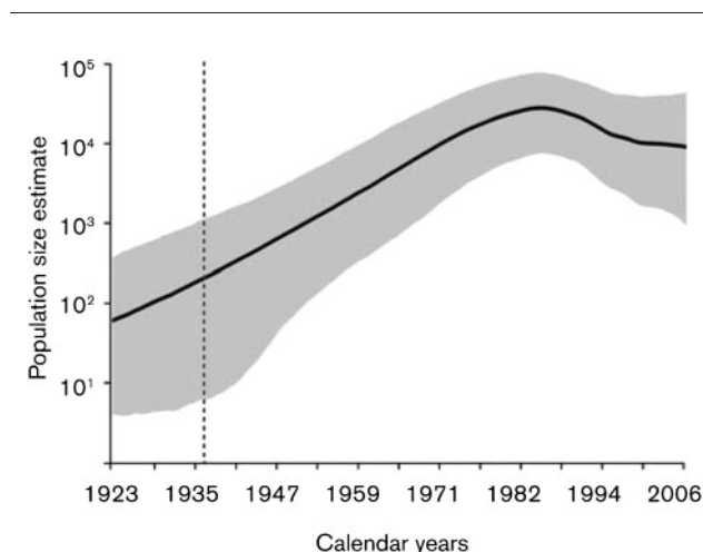
Fig. 1. The historical population dynamics of HIV-2A. Bayesian skyride analysis depicting the mean changes in effective population size ( N_e ) through time with 95% BCI for the most informative dataset (global env ).
