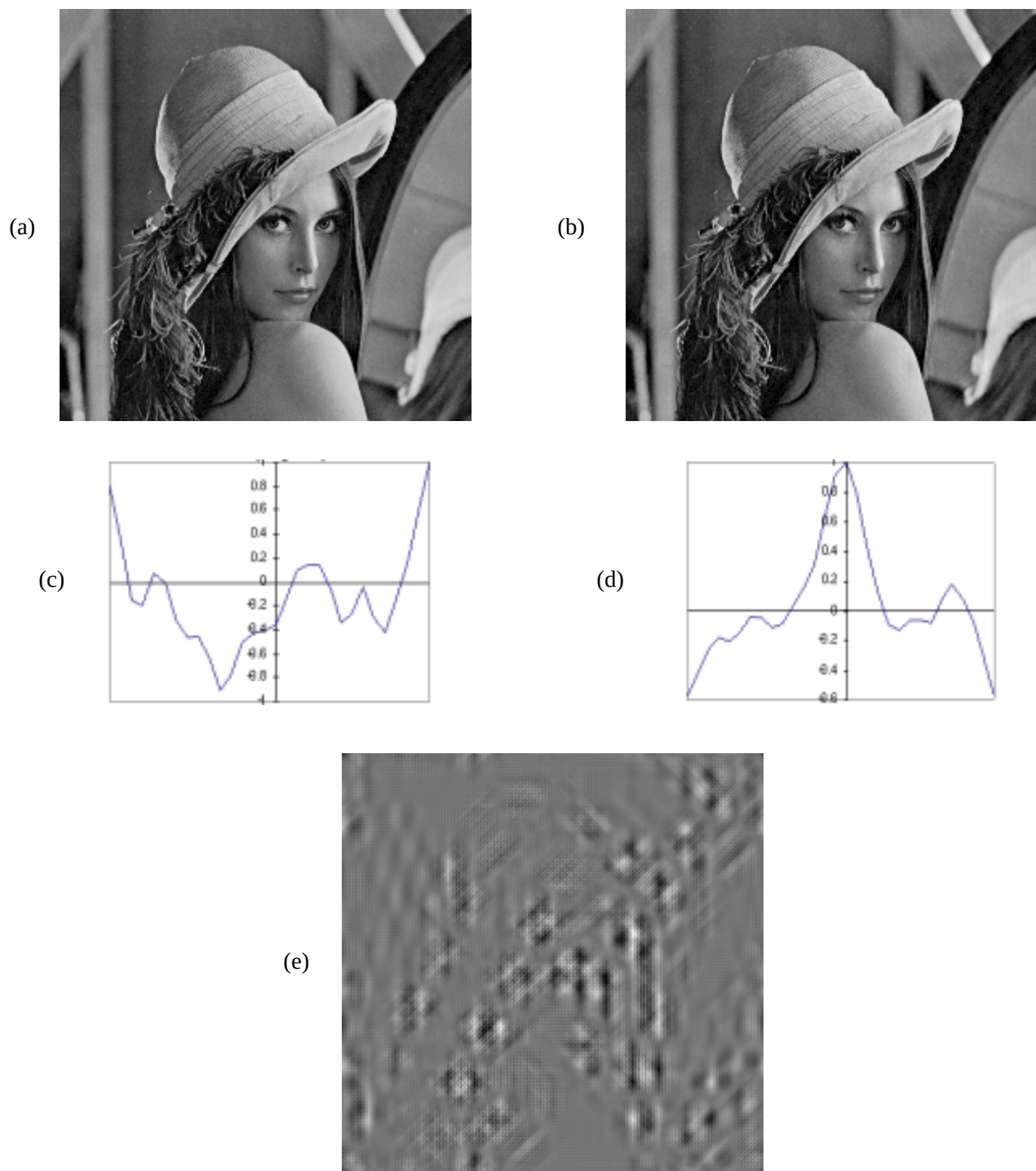
Figure 4: Results for Lena: (a) Original, (b) Watermarked one, (c) Correlation grafic for original, (d) Correlation grafic for watermarked, (e) Watermark.
