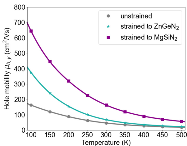
FIG. 3. Hole mobility in the y direction as a function of temperature, calculated with the full ab BTE, for unstrained GaN (gray), GaN@ZnGeN 2 (teal), and GaN@MgSiN 2 (magenta).
