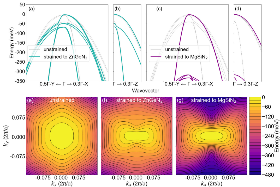
FIG. 2. (a) and (b) Valence-band structure of GaN (gray dashed lines) and GaN@ZnGeN 2 (green solid lines) near the band extremum. (c) and (d) Valence-band structure of GaN (gray dashed lines) and GaN@MgSiN 2 (purple solid lines) near the band extremum. (e) Energy of the highest valence band of GaN vs k_x and k_y in a two-dimensional plot with k_z = 0 . (f) The same setup as in (e), but for GaN@ZnGeN 2 . (g) The same setup as in (e), but for GaN@MgSiN 2 .
