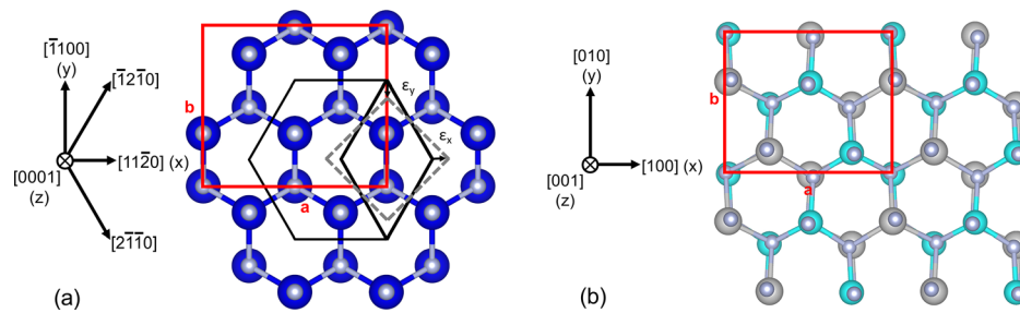
FIG. 1. (a) Crystal structure of GaN with Ga shown in dark blue and N in silver. The primitive unit cell of GaN is shown as the thick black diamond, and the orthorhombic unit cell is shown in red. The lattice parameters a and b refer to the orthorhombic cell. The deformed gray diamond shows the strain directions (not in scale). We also show how the Cartesian reference frame is aligned with respect to the standard crystallographic directions of the hexagonal lattice. (b) Crystal structure of \text{ZnGeN}_2 and \text{MgSiN}_2 with Zn or Mg shown in light blue and Ge or Si in gray. The crystallographic directions of the orthorhombic lattice are aligned with the Cartesian axis.
