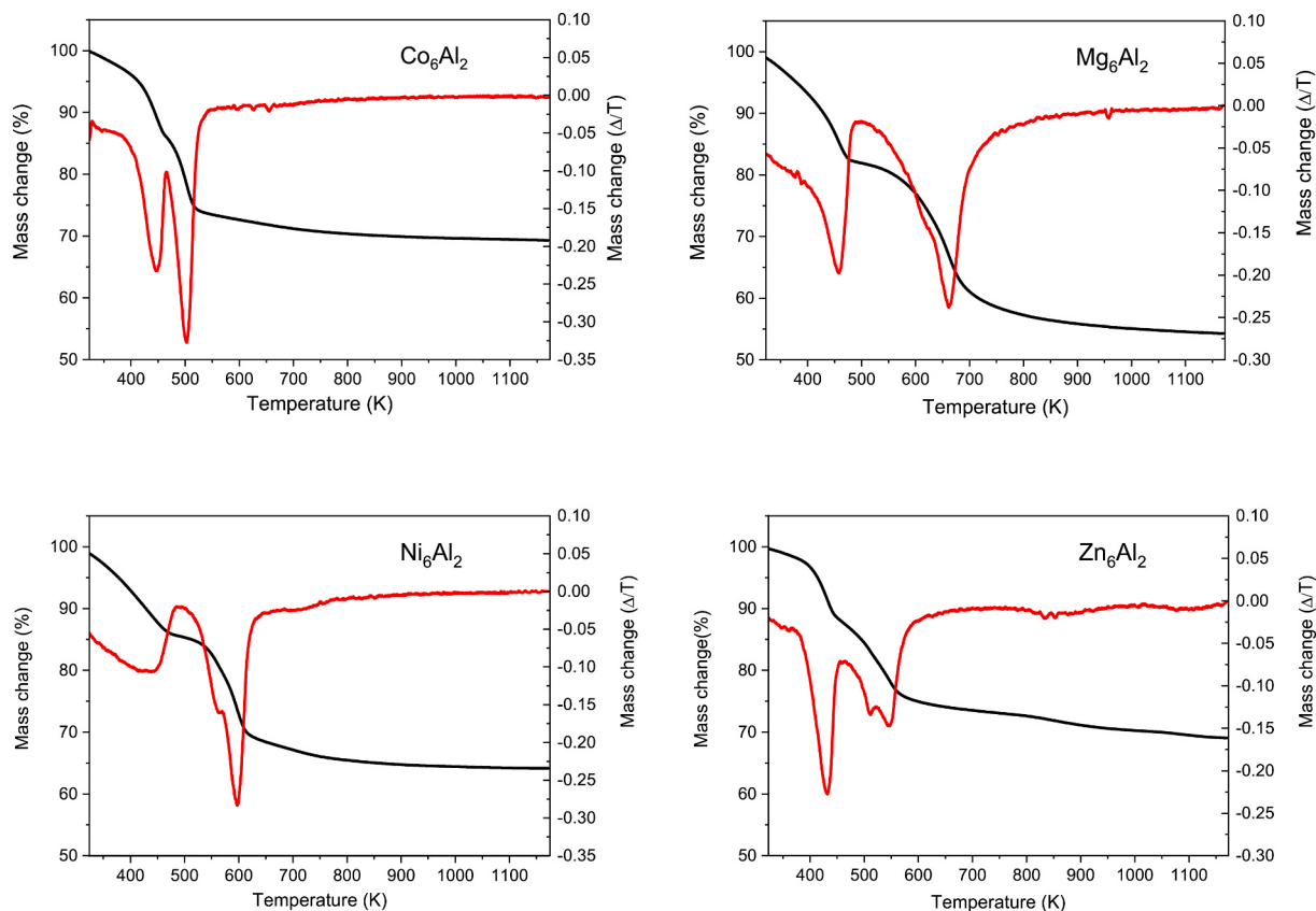
Fig. 4. TG and DTG curves of the LDH prepared with extracted aluminum.
