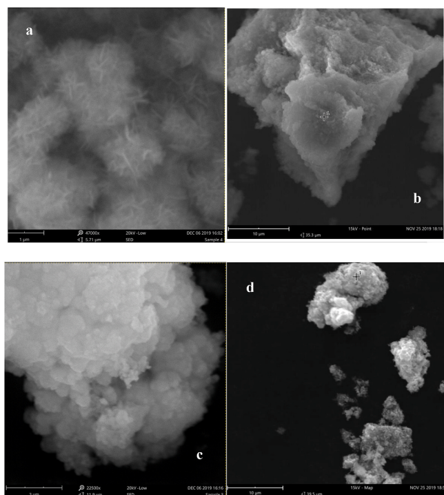
Fig. 3. SEM micrographs of the cobalt (a), magnesium (b), nickel (c) and zinc (d) samples.
