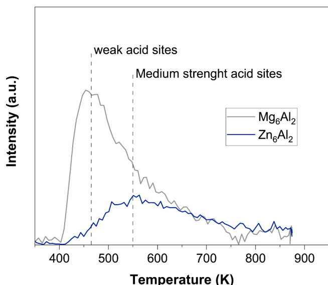
Fig. 6. NH 3 TPD patterns for Mg 6 Al 2 and Zn 6 Al 2 calcined samples.
