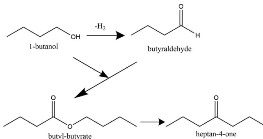
Scheme 2. 1-butanol dehydrogenation pathways.
