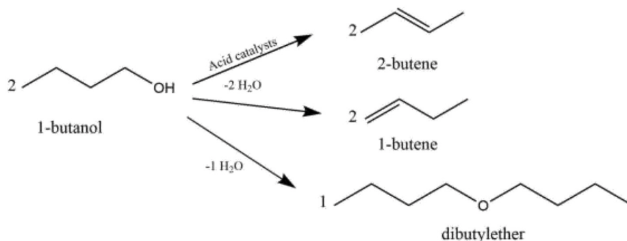
Scheme 1. 1-butanol dehydration pathways.
