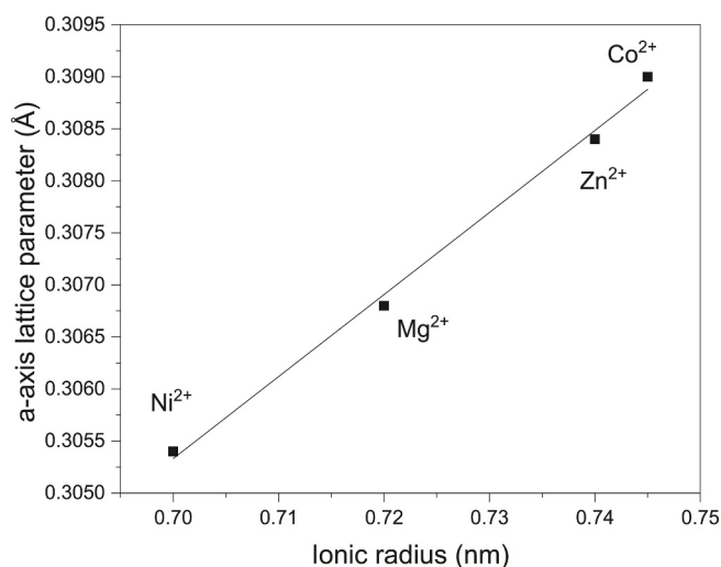
Fig. 2. Linear relationship between the dopant ionic radius and a -axis cell parameters.
