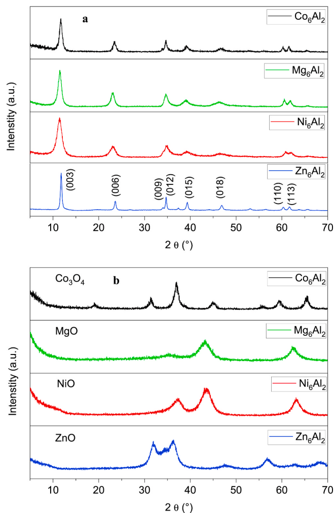
Fig. 1. Powder X-ray diffraction patterns of non-calcined (a) and calcined samples (b).
