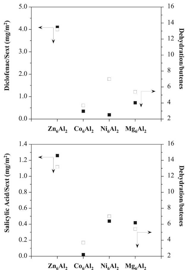
Fig. 9. Evolution of the amount of pollutants adsorbed/Seft to the butenes formation in the dehydrogenation reaction of 1-butanol. (■) pollutants, (□) dehydrogenation.
