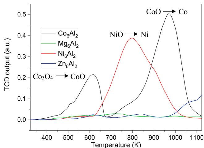
Fig. 5. \text{H}_2 -TPR profile of \text{Co}_6\text{Al}_2 , \text{Mg}_6\text{Al}_2 , \text{Ni}_6\text{Al}_2 and \text{Zn}_6\text{Al}_2 calcined samples.
