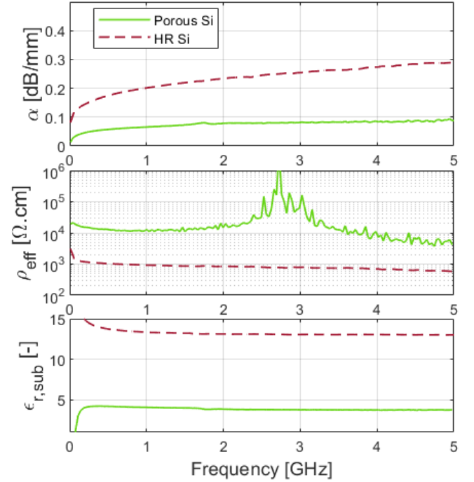
Fig. 4. Effective electrical substrate parameters extracted from wideband S-parameter measurements of RF CPW-lines at 25 °C for AlN-on-HR-Si and AlN-on-PSi Substrates. Top: CPW line losses per unit length. Middle: effective substrate resistivity. Bottom: substrate relative permittivity.
