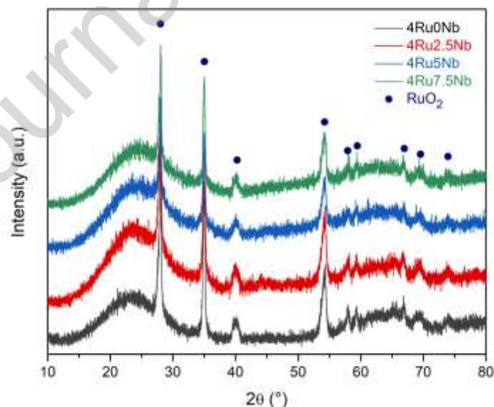
Figure 1. XRD patterns of gel-derived materials annealed at 500 ^{\circ}\text{C} for 2 h. The pattern of the corresponding 4Ru0Nb sample is also reported as a reference.
