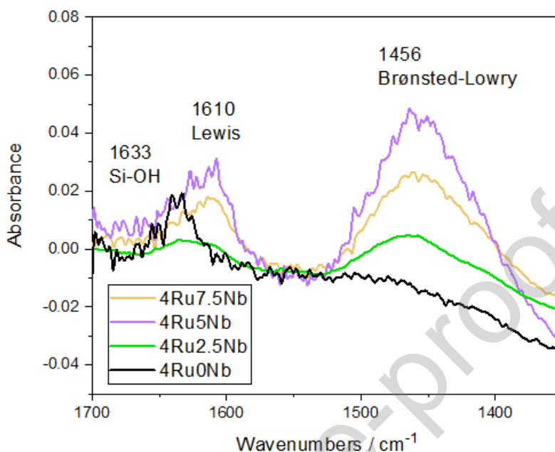
Figure 2. Difference FTIR spectra concerning the room temperature adsorption of NH 3 (equilibrium partial pressure ca 5.0 mbar) on the samples previously outgassed at 300 °C. Spectra have been normalized to sample unit weight, in order to allow comparison.
