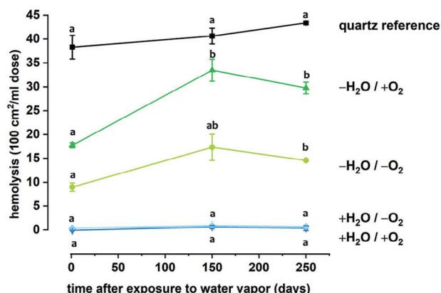
Figure 5. Membranolytic activity of the quartz (100 cm 2 ml -1 ) milled in the four different environmental conditions ( t = 0 ) and exposed to water vapor at different time points (1, 150, and 250 days). Industrial quartz was used as reference quartz because of its well-known membranolytic activity and measured at the same time points. [36,40] Values are means \pm SD and values with different letters are significantly different ( p < 0.05 ), as estimated by repeated measure one-way ANOVA with Tukey's post-hoc test.
