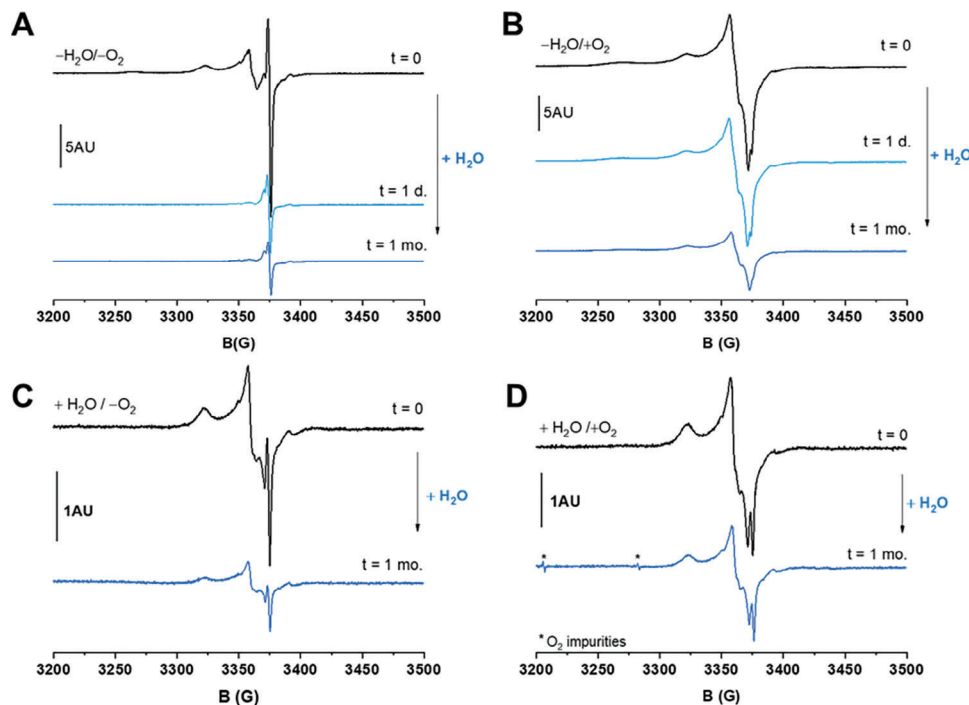
Figure 3. EPR signals of quartz milled in the four molecular environments and exposed to water vapor at different time points. Spectra of quartz milled in A) -\text{H}_2\text{O}/-\text{O}_2 , B) -\text{H}_2\text{O}/+\text{O}_2 , C) +\text{H}_2\text{O}/-\text{O}_2 , and D) +\text{H}_2\text{O}/+\text{O}_2 before ( t = 0 ) and after exposure to 25 mbar of \text{H}_2\text{O} vapor for t = 1 day and 1 month are recorded at 77 K after degassing the EPR cell.
