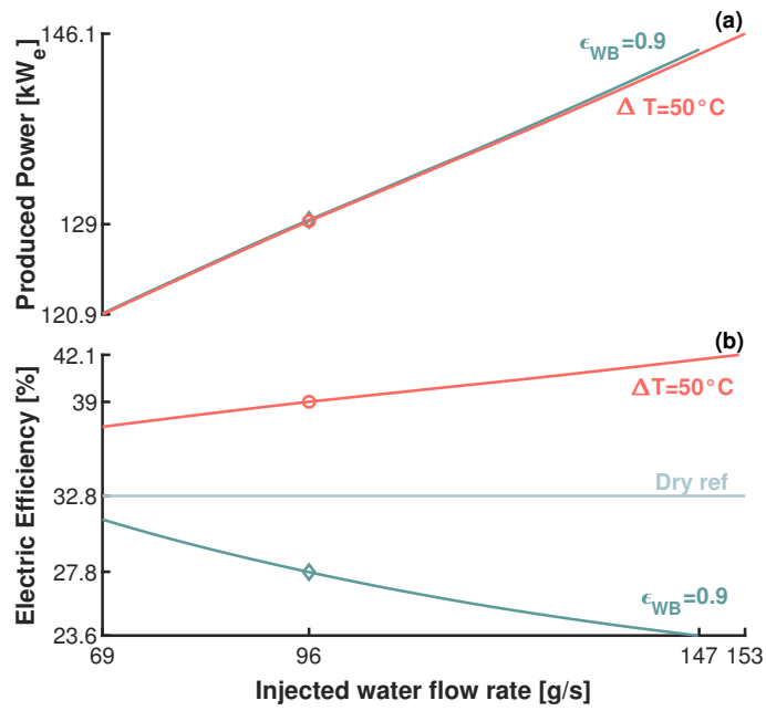
Figure 3: Performance results of the M-power cycle, using different assumptions on the M-power saturator performance, indicate that by maximizing the waste heat recovery only ( \Delta T = 50^\circ\text{C} case), both electric power output (a) and efficiency (b) can be improved.
