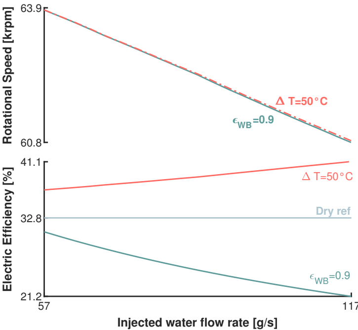
Figure 5: Similar to operation at constant rotational speed, at constant power output (100 kW e ), the performance of the M-power cycle can only be improved by maximizing the waste heat recovery ( \Delta T = 50^\circ\text{C} case), and while doing so, increasing the electric efficiency.
