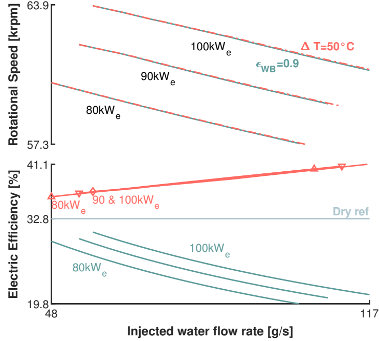
Figure 13: The requested power output has no impact on the global electric performance, when assuming a constant hot pinch ( \Delta T = 50^\circ\text{C} ).
