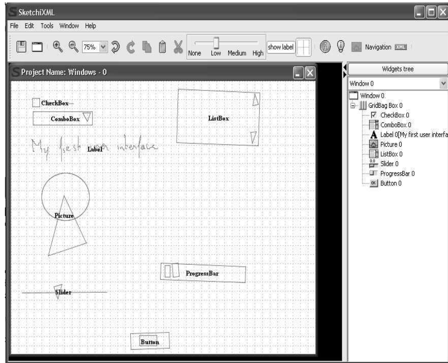
Figure 7.5 A general screen shot of the sketching tool
