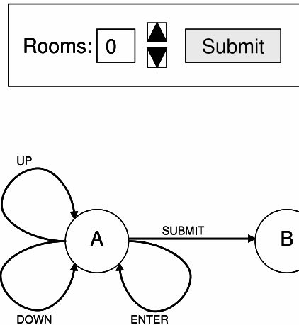
Figure 7.10 Room reservation form and corresponding state machine.
