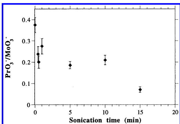
Figure 4. Evolution of the \text{PrO}_3^-/\text{MoO}_3^- intensity ratio in C-type \text{Pr}_6\text{O}_{11} - \text{MoO}_3 mixtures (Pr/Mo = 6) as a function of the sonication time.
