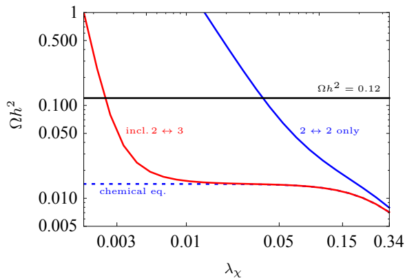
FIG. 4. Relic density as a function of the coupling \lambda_\chi , for m_\chi = 100 GeV, m_{\tilde{t}} = 110 GeV. The red line shows the solution including the 2 \leftrightarrow 3 conversion processes, the blue line corresponds to the solution when only 2 \leftrightarrow 2 conversion processes (and decays) are considered. The dotted blue line is the result that would be obtained when assuming chemical equilibrium.
