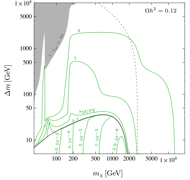
FIG. 1. Viable parameter space in the plane spanned by m_\chi and \Delta m = m_{\tilde{t}} - m_\chi . For each point we adjust \lambda_\chi such that \Omega h^2 = 0.12 . Above the thick black curve chemical equilibrium holds (WIMP region), while below this curve chemical equilibrium breaks down and solutions for the conversion-driven freeze-out exist. The green solid curves denote contours in the coupling \lambda_\chi . For comparison, the black dotted curve shows the allowed parameter slice for a realization of a super-WIMP scenario within the model (see comment at the end of Sec. III B).
