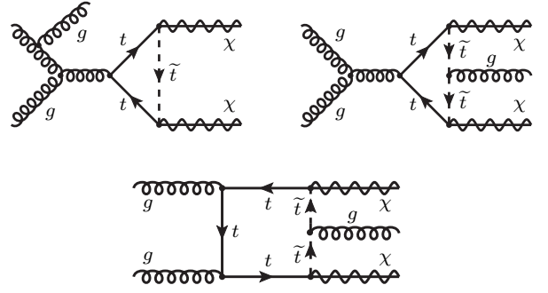
FIG. 7. Representative Feynman diagrams for the process pp \rightarrow \chi\chi + j with up to five internal (s)top legs.
