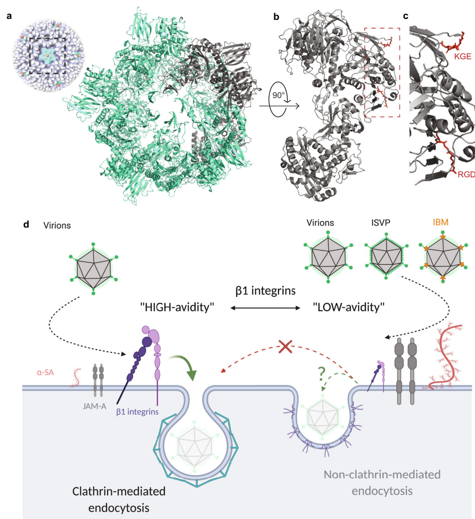
Fig. 7 Integrin interaction with λ2 reovirus outer capsid protein mediates clathrin-recruitment for entry into host cells. a Crystal structure of the λ2 turret (pentamer, about 120 Å diameter and 80 Å tall), viewed from the top. Cryo-electron microscopy reconstruction of the virion is shown on the side 8,55 . The five elongated λ2 monomers, four shown in green and one in gray, wrap around the other surface, with their long axes about 45° to the radial direction. b The λ2 monomer, viewed from the side (the gray monomer in a ). β1 integrin binding sequences, RGD and KGE, are highlighted as red sticks. c Zoom-in on β1 integrin binding domain in λ2. Images are based on related crystal structure 1EJ6 [ https://doi.org/10.1038/35010041 ]. d Conclusive model: Virions efficiently bind β1 integrins ("high-avidity" binding), which mediates recruitment of clathrin for virus internalization. Virions in the presence of abundant free α-SA or ISVPs bind poorly to integrins ("low-avidity" binding), potentially because of steric hindrance from conformational changes in σ1. Consequently, they use alternate mechanisms for entry such as caveolin-mediated endocytosis, similar to virions lacking the β1 integrin domain (IBM).
