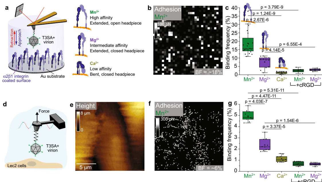
Fig. 2 Reovirus directly engages \beta 1 integrins in a cation-dependent manner. Studies were conducted using model surfaces ( a–c ) and living cells ( d–g ). a Experimental set up (left) to probe cation-dependent (right) virion- \alpha 2\beta 1 integrin interactions using a model surface. b The adhesion map shows interaction forces (white pixels) between virions and integrins in the presence of Mn^{2+} , which induces an extended integrin conformation. c Box plot of specific binding frequencies (BF) measured using AFM between virions and integrins in the presence of divalent cations and following injection of cRGD. d FD-based AFM setup to study T3SA+ binding to Lec2 cells, which express \beta 1 integrins. Height ( e ) and corresponding adhesion maps ( f ) of the imaged area show specific binding of reovirus T3SA+ to living Lec2 cells in the presence of Mn^{2+} (white pixels). For better visibility, the pixel size in the adhesion image was enlarged two-fold. AFM images were acquired using an oscillation frequency of 0.25 kHz and amplitude of 750 nm under cell culture conditions. g Box plot shows BF of T3SA+ virions to \beta 1 integrins on living Lec2 cells under conditions shown. The horizontal line within the box indicates the median, boundaries of the box indicate the 25th and 75th percentile, and whiskers indicate the highest and lowest values. Open square within each box indicates the mean. All data are representative of N = 5 independent experiments. P values were determined by two-sample t -test using Origin.
