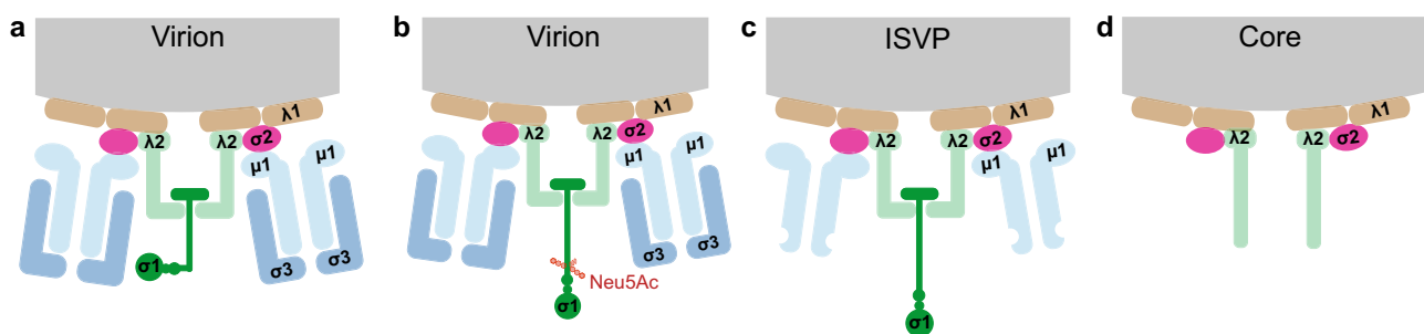
Fig. 1 Schematic of capsid composition of reovirus particles. a–d Diagrams of cross-sections of reovirus virions, infectious subviral particles (ISVPs), and cores. Schematics depict the arrangement and conformation of structural proteins in the double-layered shells of the virions in the absence (a) and presence (b) of Neu5Ac (triggering a conformational change of \sigma 1 ); removal of \sigma 3 , cleavage of \mu 1 , and rearrangement of \sigma 1 in ISVPs (c); and removal of \mu 1 fragments, loss of \sigma 1 , and opening of the \lambda 2 turret in cores (d).
