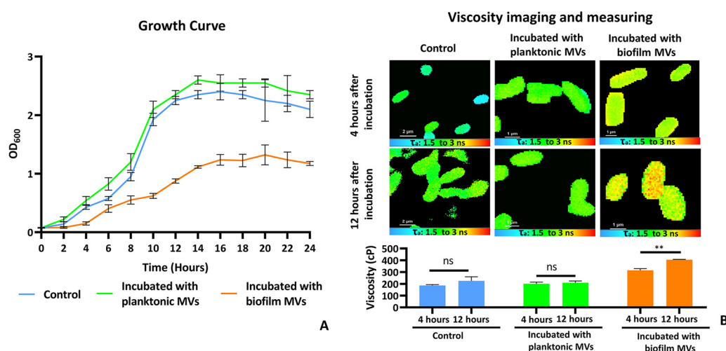
FIG 5 Growth curves of P. aeruginosa in the presence of MVs and the effect of incubation with MVs on membrane fluidity of P. aeruginosa . (A, left) Growth curves of the bacterial control culture (nonsupplemented medium), medium supplemented with MVs of the planktonic P. aeruginosa , and medium supplemented with MVs of the biofilm P. aeruginosa . (Top, right) FLIM images of planktonic P. aeruginosa in unsupplemented medium (control), medium supplemented with MVs of the planktonic bacteria, and medium supplemented with MVs of the biofilm bacteria after 4 h of incubation. (Middle) After 12 h of incubation. (Bottom) Calculated viscosity corresponding to the upper panels, according to the lifetime of BODIPY-C10. (B) The data were obtained from two individual experiments, and in each experiment, at least 10 bacteria or three slides were considered for measuring the lifetimes of the bacteria. The data are presented as means \pm SD from independent replicates under each condition. Statistical analysis was performed by paired t test. **, P < 0.01 ; ns, not significant.
