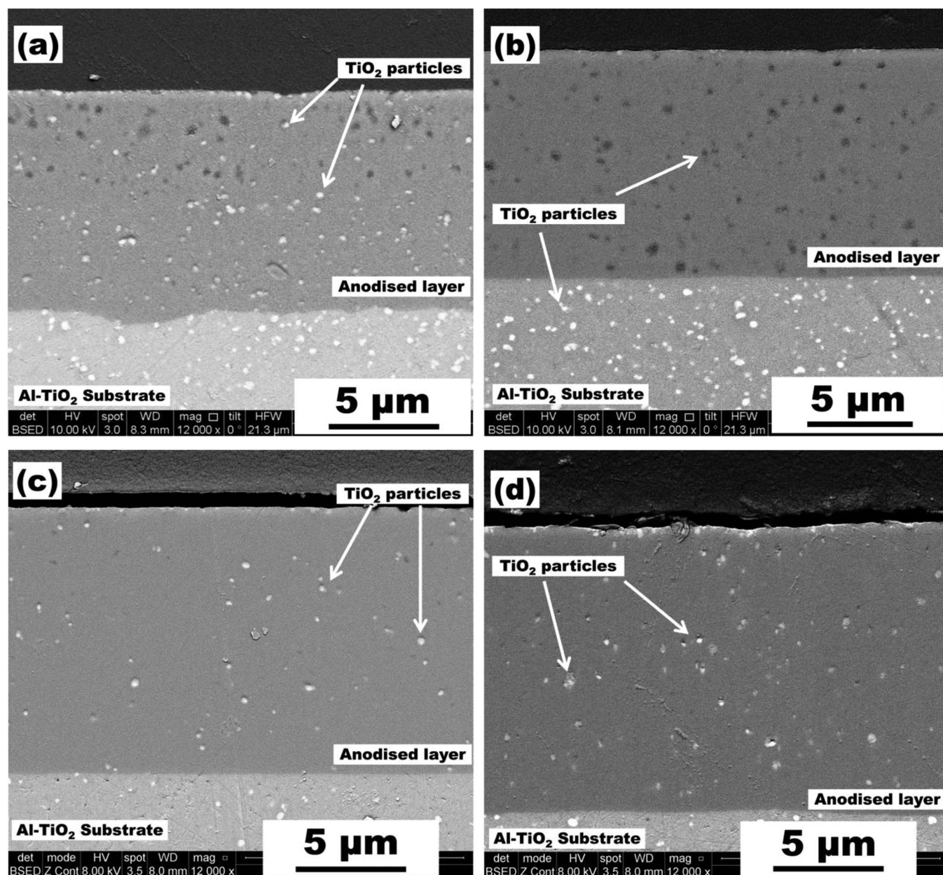
Figure 4. SEM-BSE cross-section image of the FSP Al-TiO 2 sample anodized using: (a) PRPA-10 V, (b) PRPA-20 V, (c) PA-10 V, and (d) PA-20 V at 2 kHz. (The TiO 2 particles can be seen in the Al-TiO 2 composite substrate and also in the anodized layer as both bright and dark spots.)
