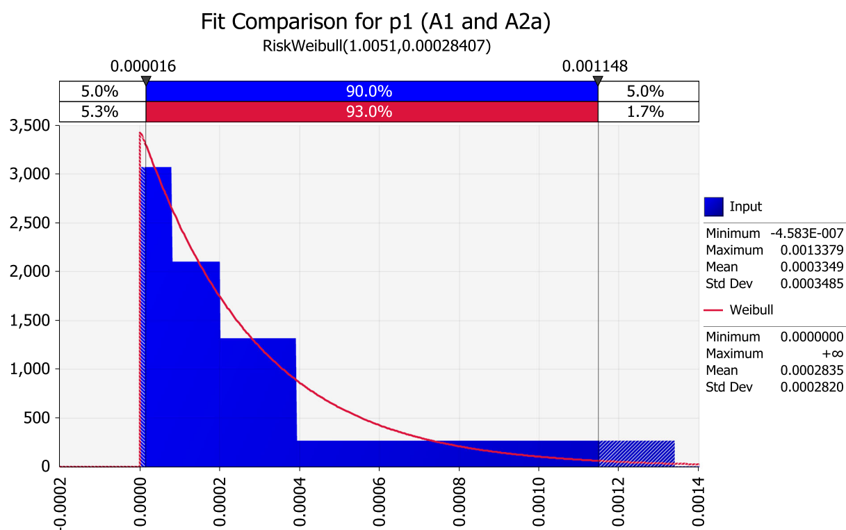
Figure 8: Fitted distribution for prevalence at the origin ( p_1 ) under scenarios A1 and A2a (one mandatory field inspection at the origin)
