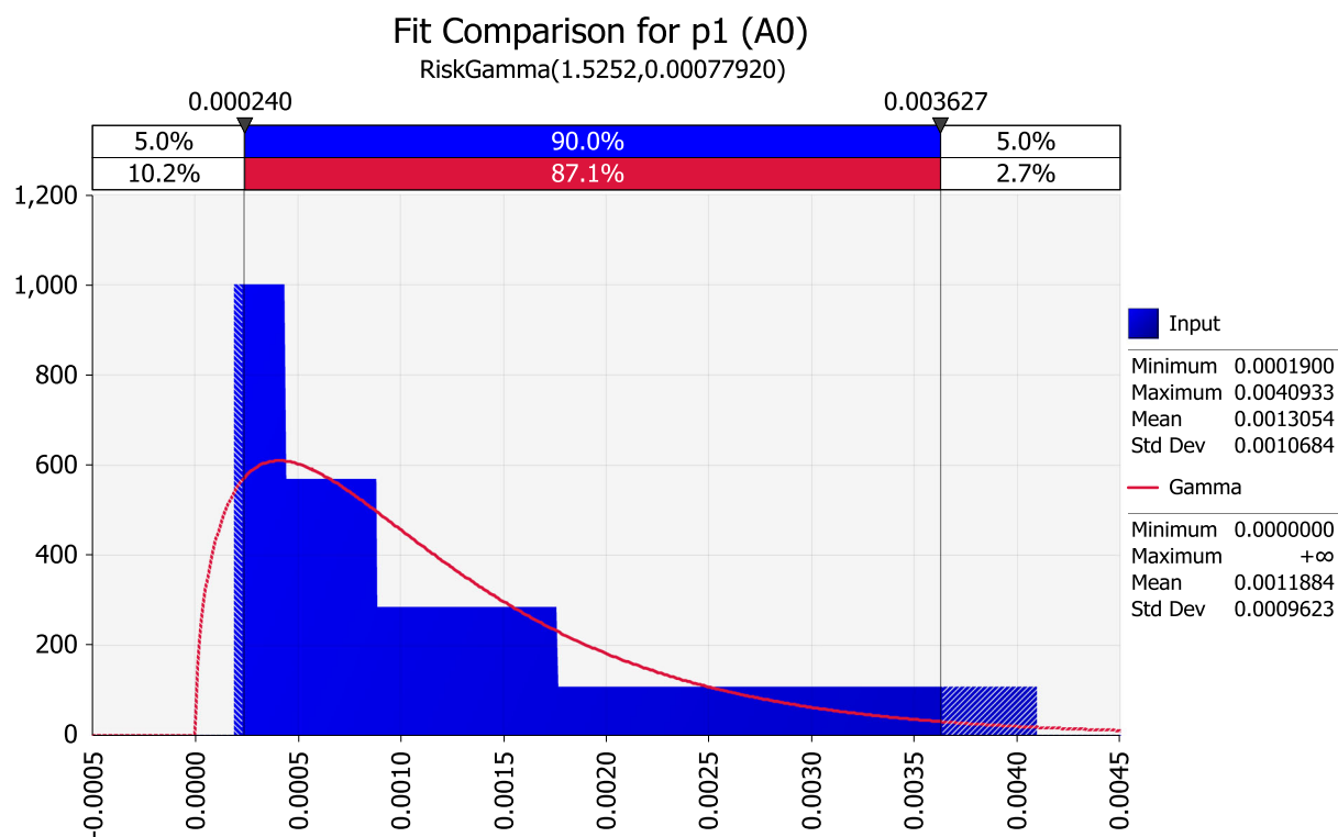
Figure 7: Fitted distribution for prevalence at the origin ( p_1 ) under scenario A0
