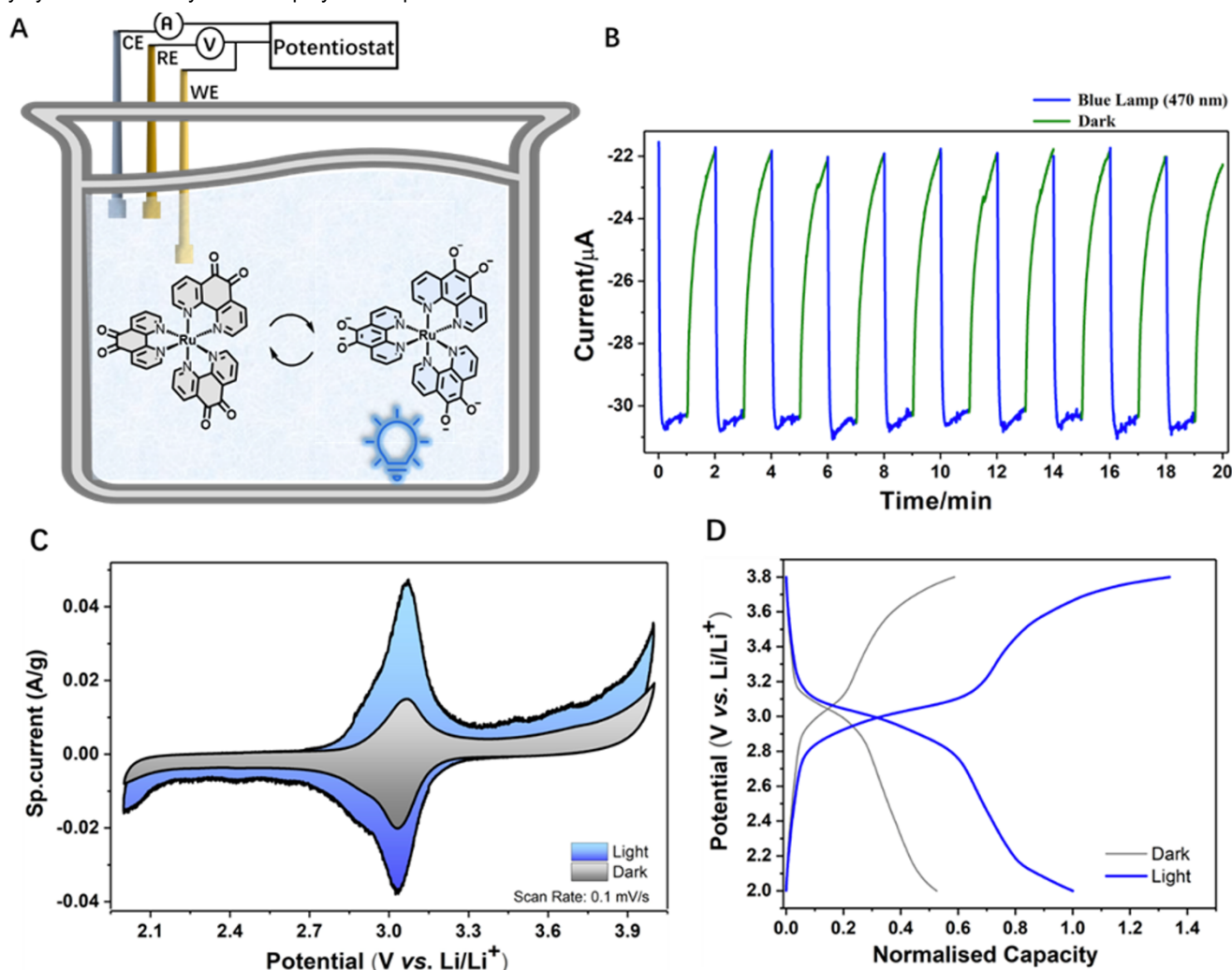
Figure 3: A) Schematic representation of potentiostatic photo-oxidation setup (concentration of 1 .PF 6 : 1 mM; WE: Glassy carbon, CE: Pt wire, RE: Ag/Ag + , electrolyte: 0.1M Tetrabutylammonium perchlorate in ACN). B) Photocurrent response to on/off irradiation conditions ( \lambda = 470 nm, intensity \sim 4.0 mW cm -2 ). C) Solid state cyclic voltammetric response (at 0.1 mV/s) and D) galvanostatic charge-discharge profiles of 2 .Li 4 (D) at 5 mA g -1 of the photo-batteries under dark and illumination ( \lambda \sim 455 nm, intensity \sim 12 mW cm -2 ) conditions, where capacities are normalized by absolute discharged capacity obtained under light.
