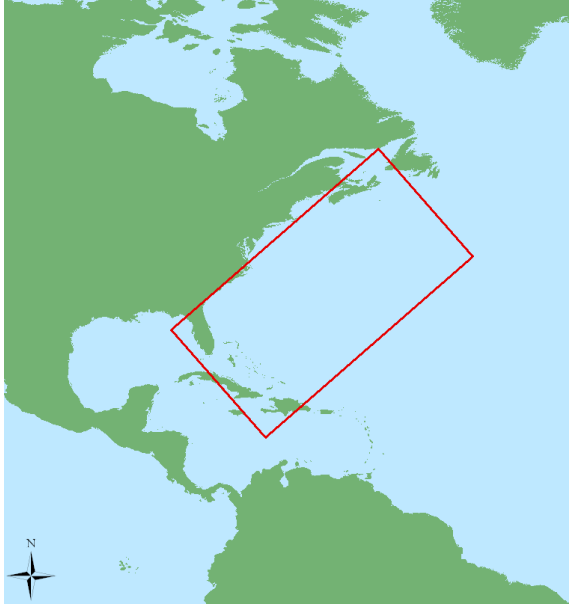
Figure 8.2 — GYRE domain (illustrated with ArcGIS™).
