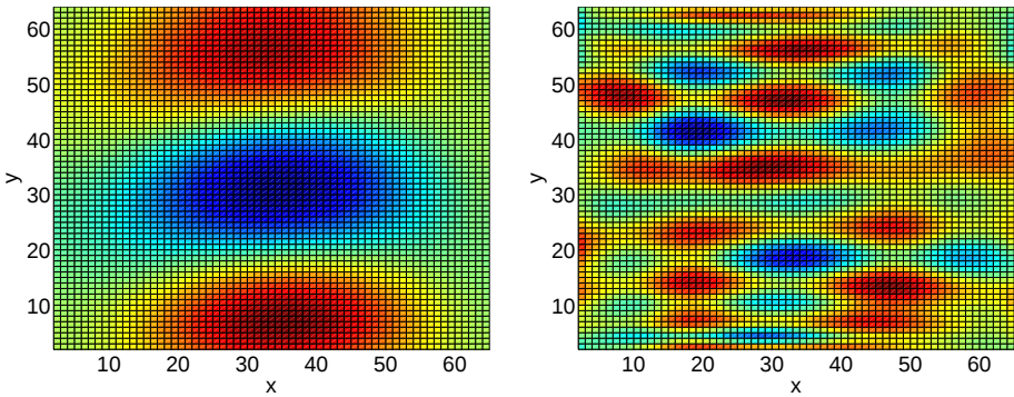
Figure 7.6 — EOF number 1 (left) and EOF number 20 (right) .
