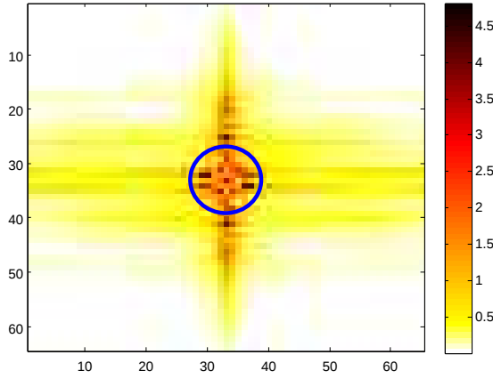
Figure 7.7 — EOF number 20 in the frequency domain.
