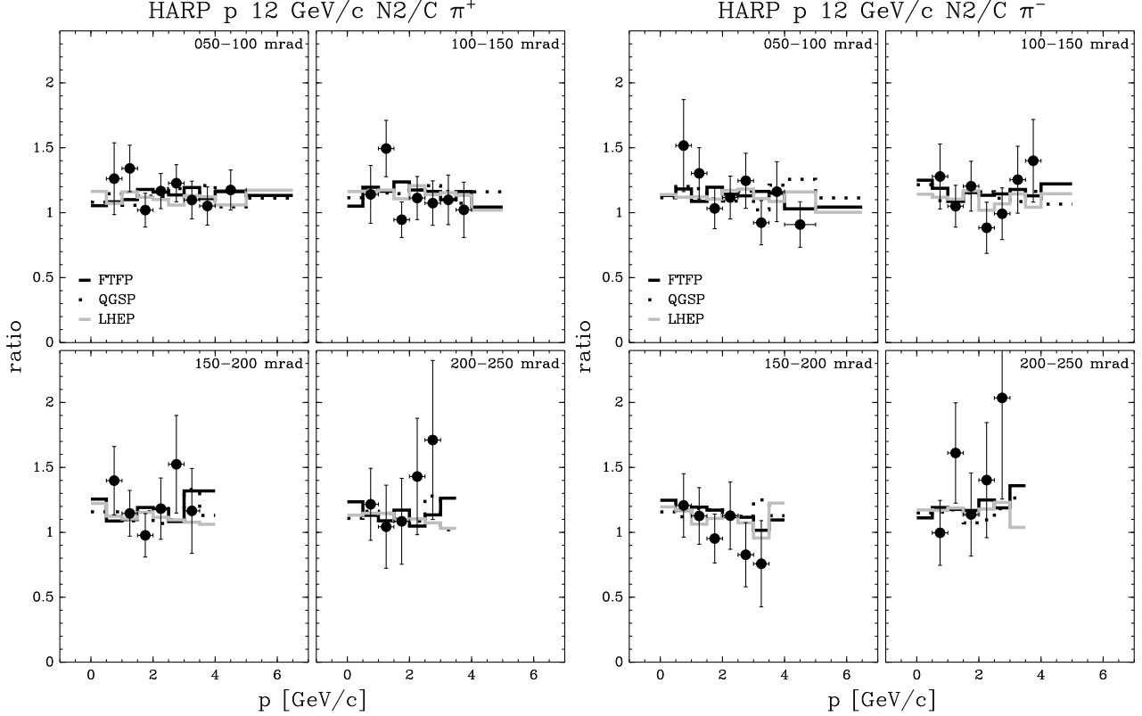
Figure 3: p -N 2 to p -C production ratio for \pi^+ (left panel) and \pi^- (right panel) at 12 GeV/ c , compared with GEANT4 simulation predictions using different models. In the top right corner of each plot the covered angular range is shown in mrad. Only statistical errors are used, since most systematic ones cancel.
