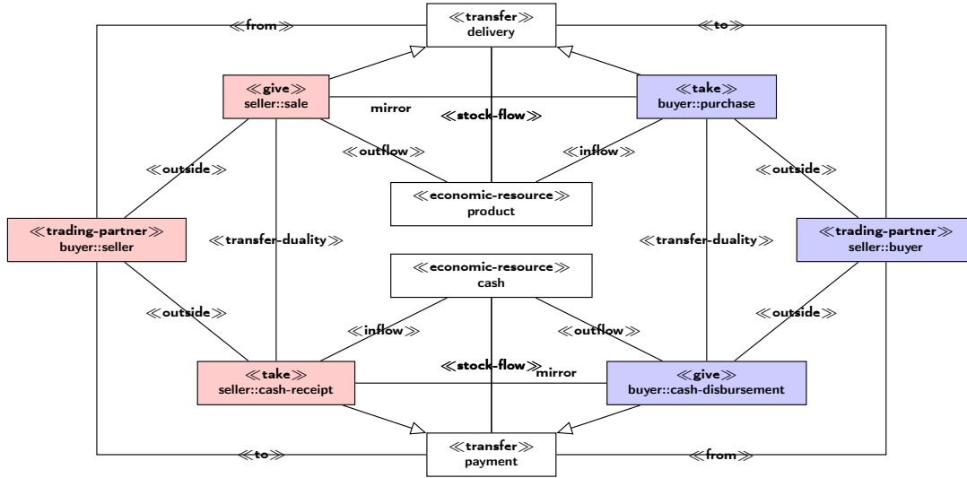
Fig. 5. Collaboration space semantics
