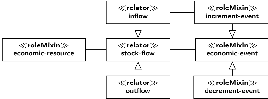
Fig. 2. The REA 2 meta-model for stock-flows
