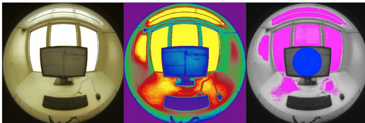
Fig. 2. Example of HDRi constructed from the seven LDRIs captured using the CCD camera ( left ); False colour Photosphere luminance map with Radiance image formatting ( centre ); Evalglare image with a blue circle at the centre of the screen representing the point of visual fixation. Pixels highlighted in pink surrounding the screen represent identified glare sources ( right ). (For interpretation of the references to colour in this figure legend, the reader is referred to the Web version of this article.)
