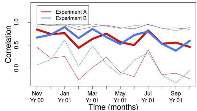
Fig. 5. Time correlation of the two experiments with the observational reference. The thick lines represent the correlation of the ensemble-mean with the references. The confidence intervals are plotted with a thinner line of the same colour.
