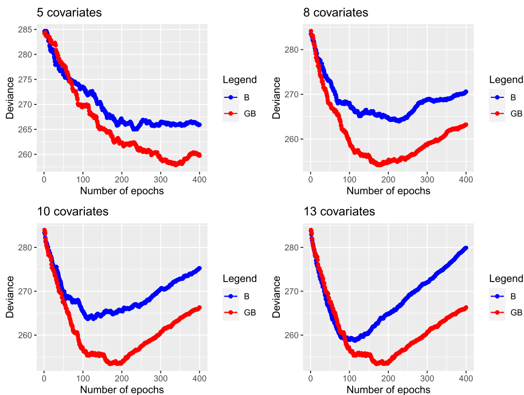
Figure 8. Claims severity: comparison of out-of-sample deviances obtained with boosting (B) and gradient boosting (GB).
