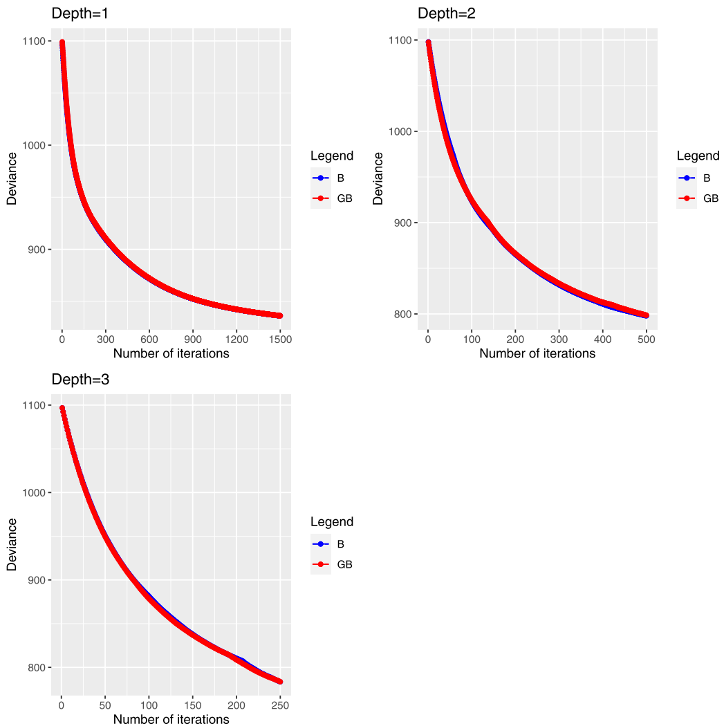
Figure 3. Claims severity: comparison of in-sample deviances obtained with boosting trees (B) and gradient boosting trees (GB).
