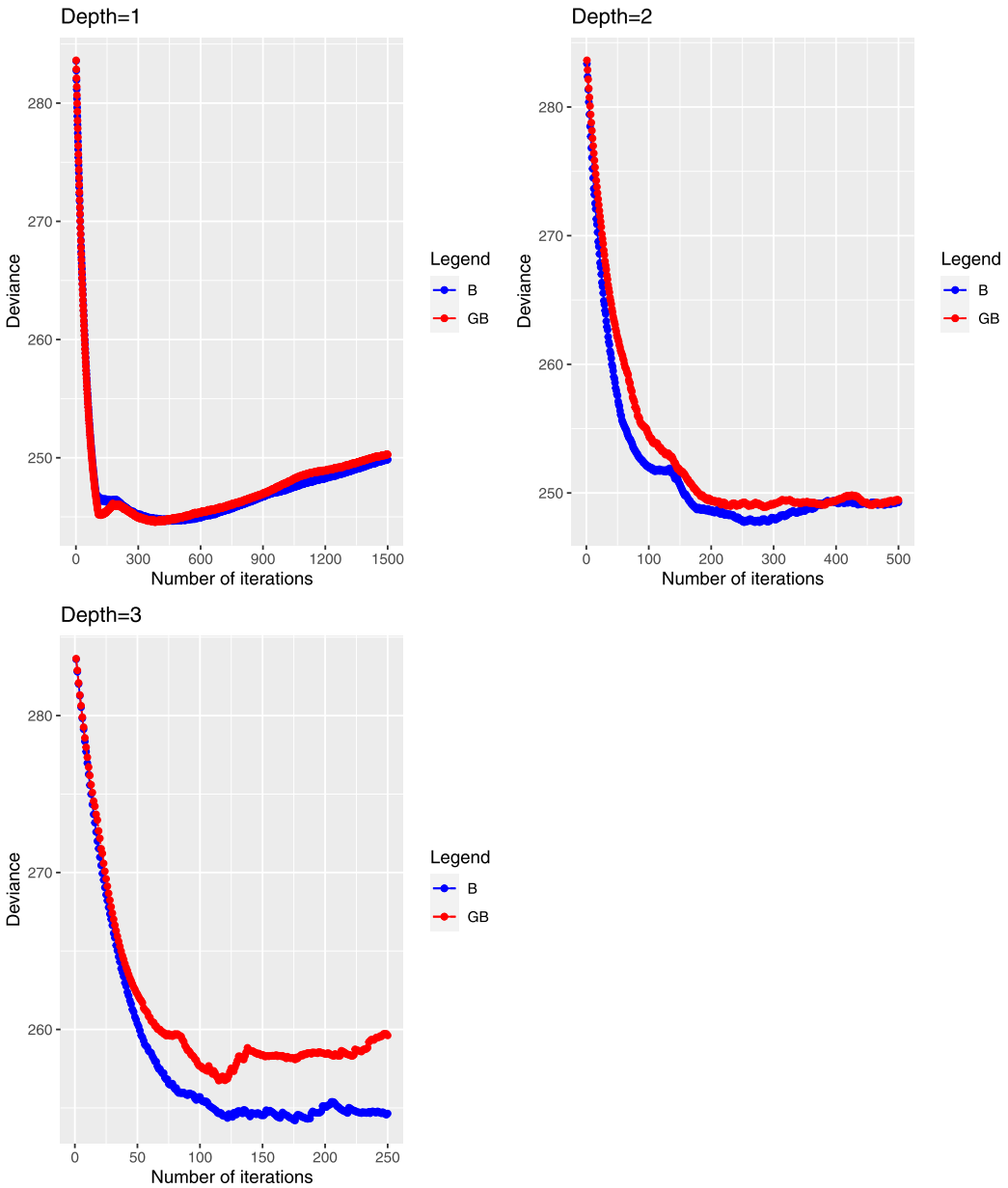
Figure 4. Claims severity: comparison of out-of-sample deviances obtained with boosting trees (B) and gradient boosting trees (GB).
