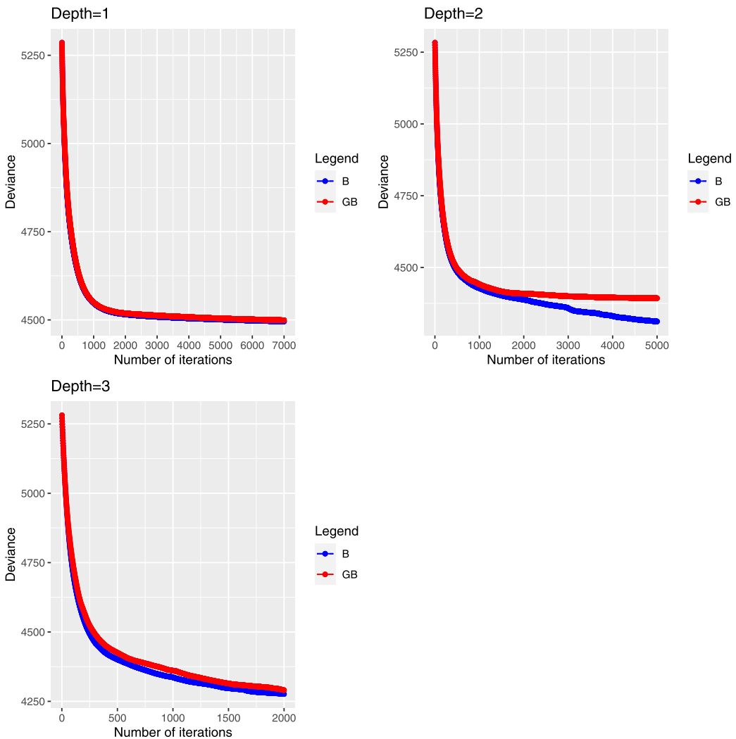
Figure 1. Claims frequency: comparison of in-sample deviances obtained with boosting trees (B) and gradient boosting trees (GB).
