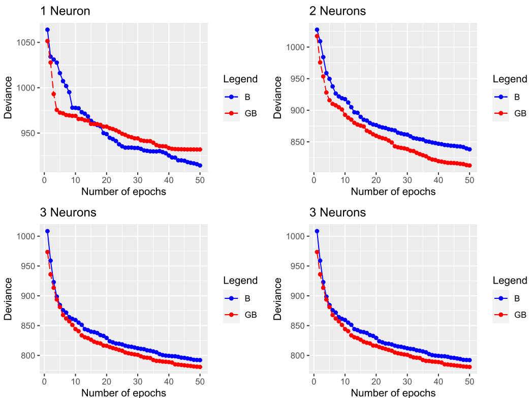
Figure 12. Claims severity: comparison of in-sample deviances obtained with boosting (B) and gradient boosting (GB).
