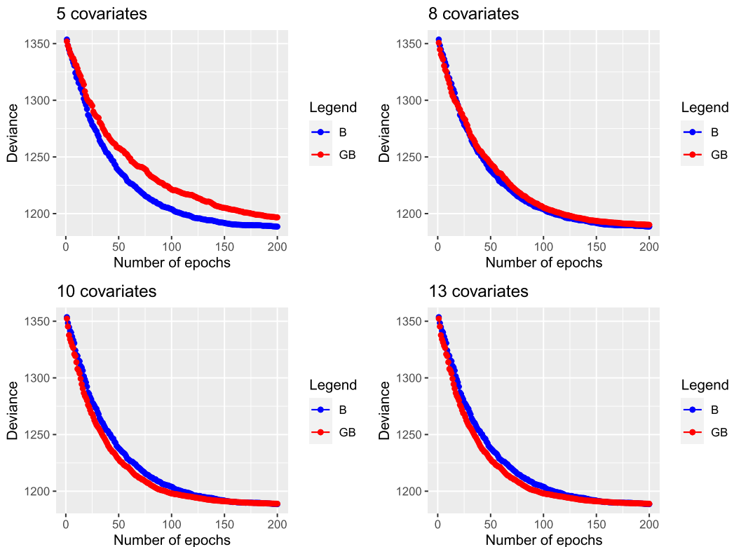
Figure 6. Claims frequency: comparison of out-of-sample deviances obtained with boosting (B) and gradient boosting (GB).
