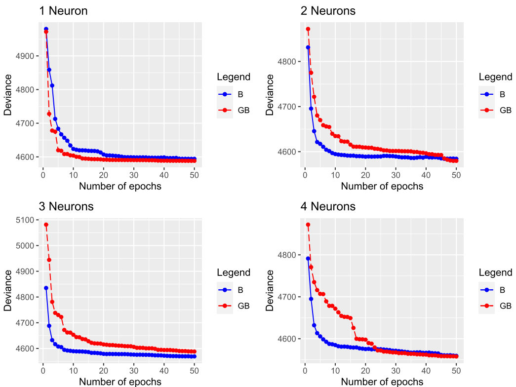
Figure 10. Claims frequency: comparison of in-sample deviances obtained with boosting (B) and gradient boosting (GB).
