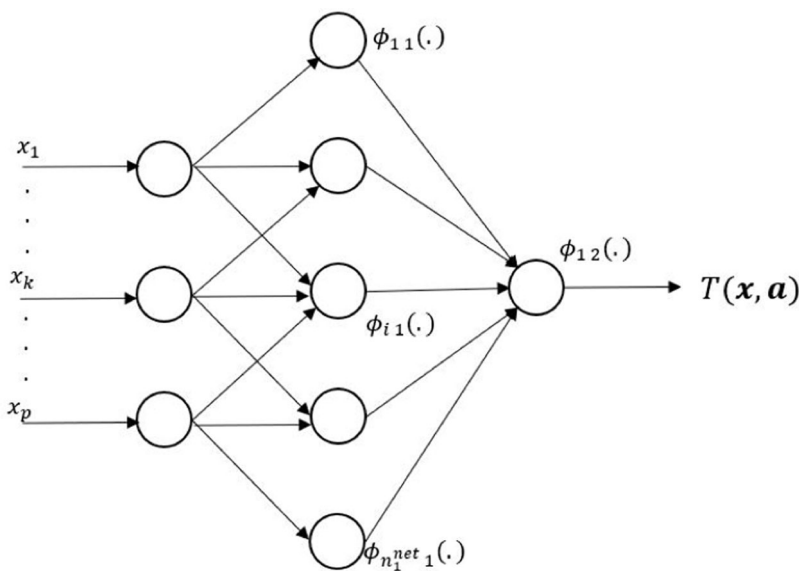
Figure 9. Illustration of a shallow neural network used as base learner in the Boosting algorithm.
