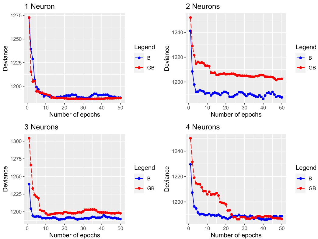
Figure 11. Claims frequency: comparison of out-sample deviances obtained with boosting (B) and gradient boosting (GB).
