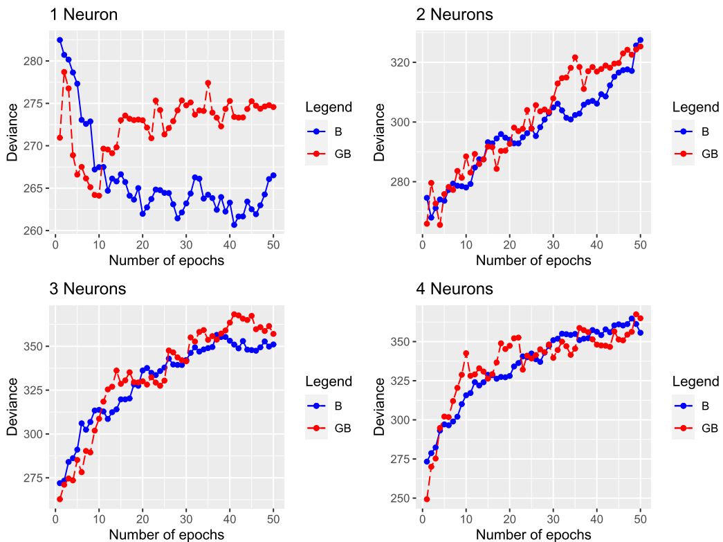
Figure 13. Claims severity: comparison of out-sample deviances obtained with boosting (B) and gradient boosting (GB).
