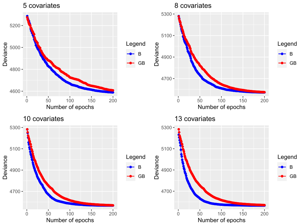
Figure 5. Claims frequency: comparison of in-sample deviances obtained with boosting (B) and gradient boosting (GB).
