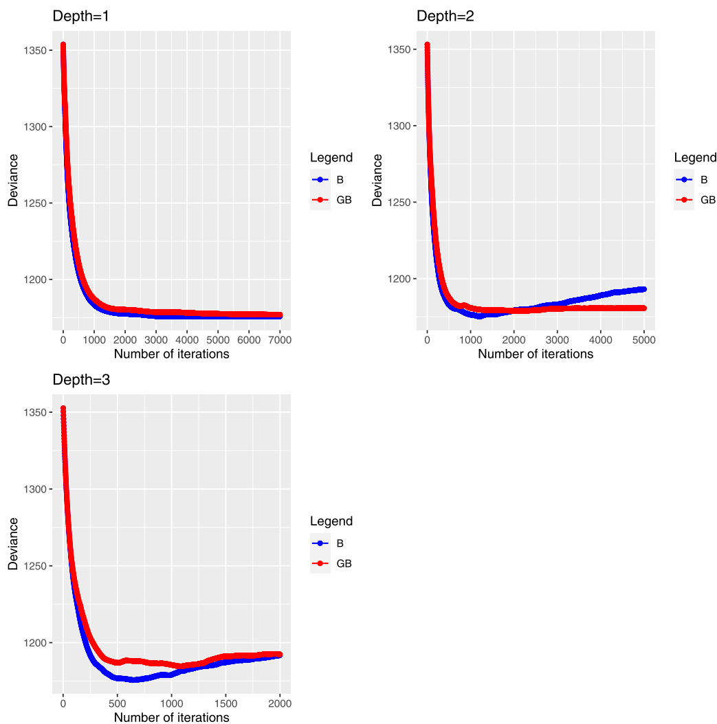
Figure 2. Claims frequency: comparison of out-of-sample deviances obtained with boosting trees (B) and gradient boosting trees (GB).
