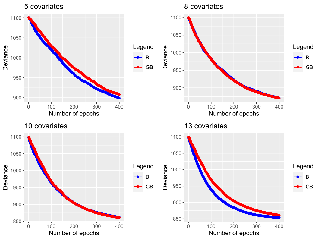
Figure 7. Claims severity: comparison of in-sample deviances obtained with boosting (B) and gradient boosting (GB).
